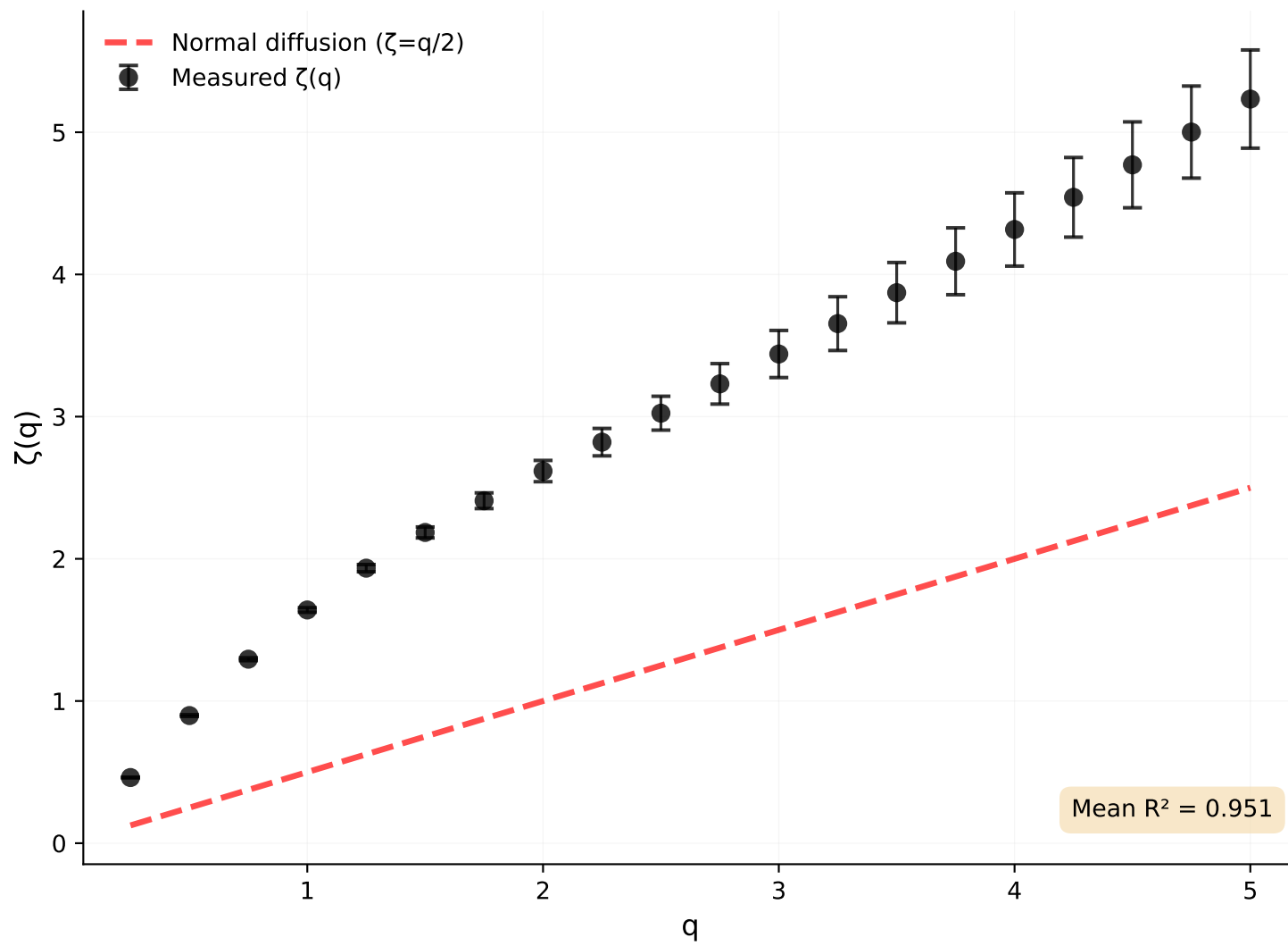
S-wave
