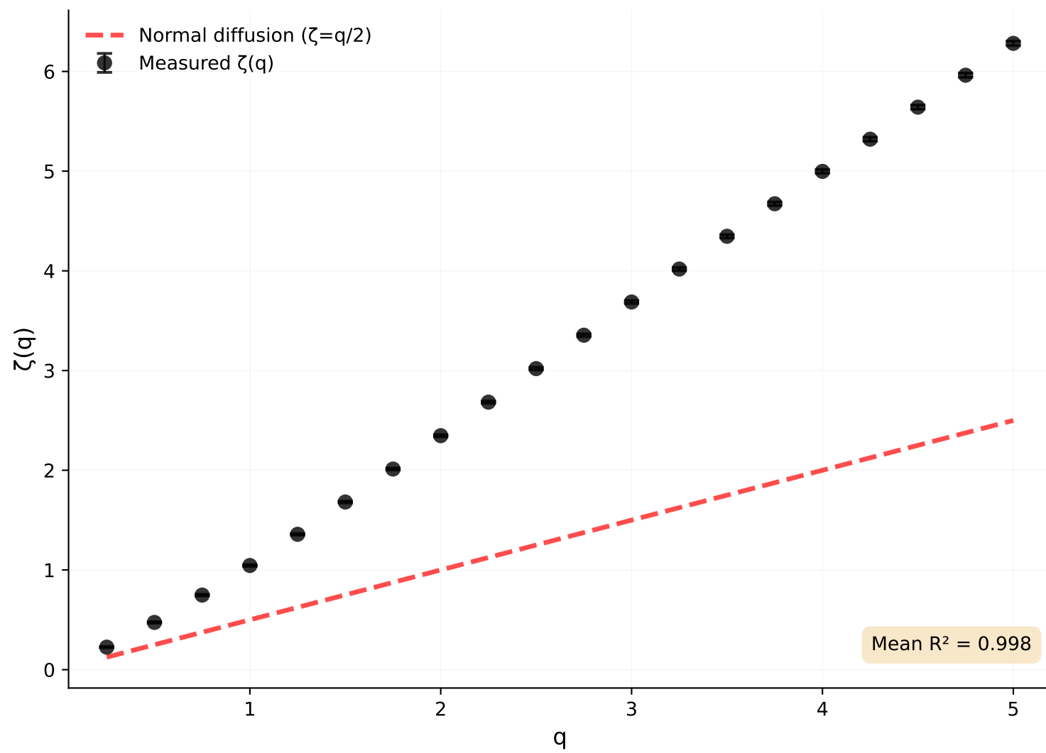
S-wave
