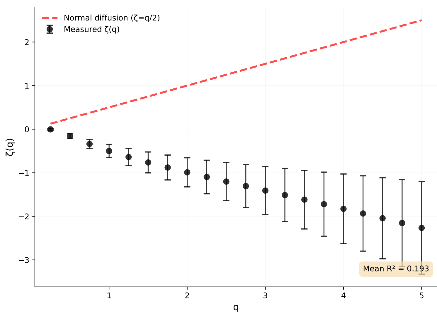
S-wave
