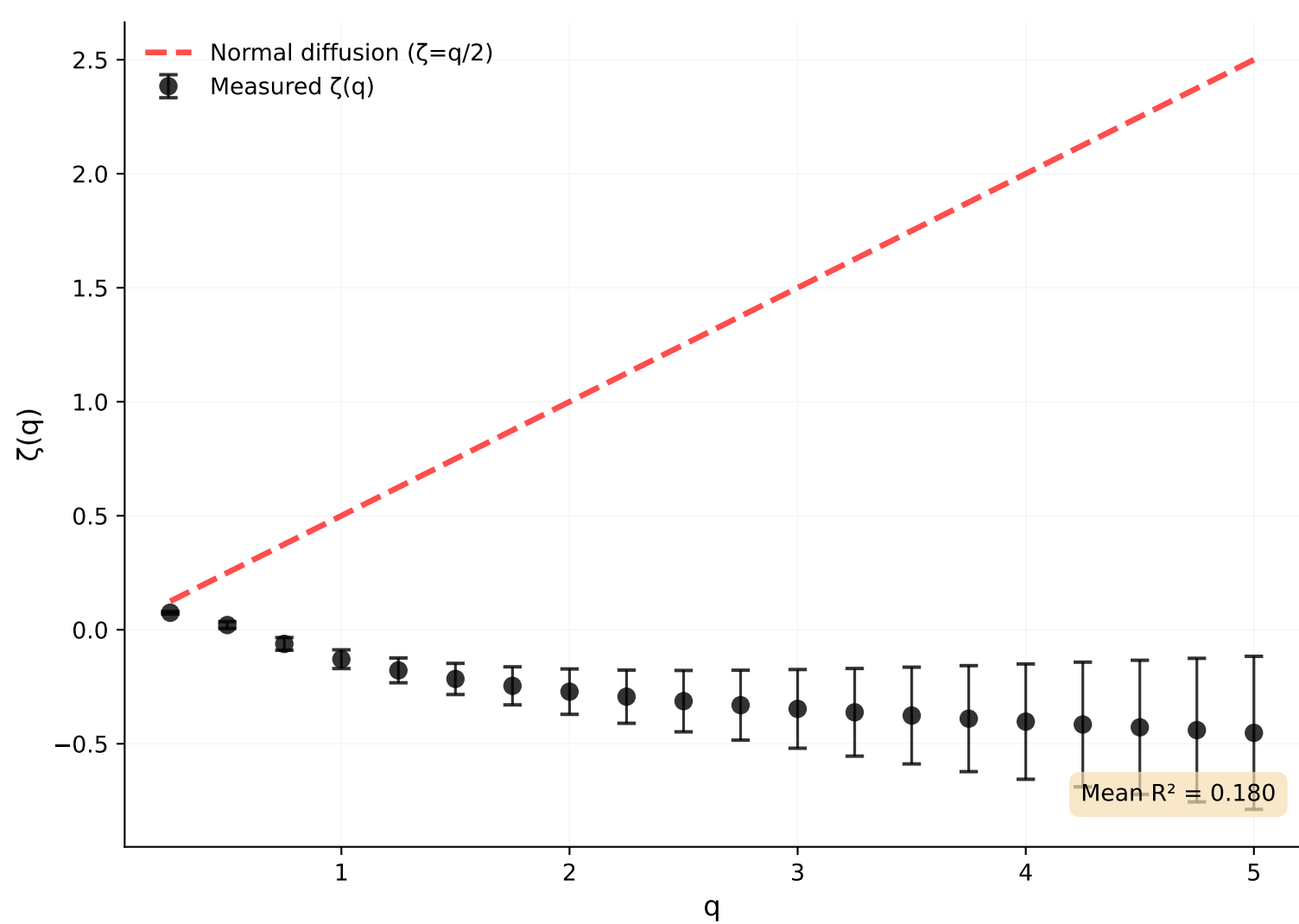
S-wave
