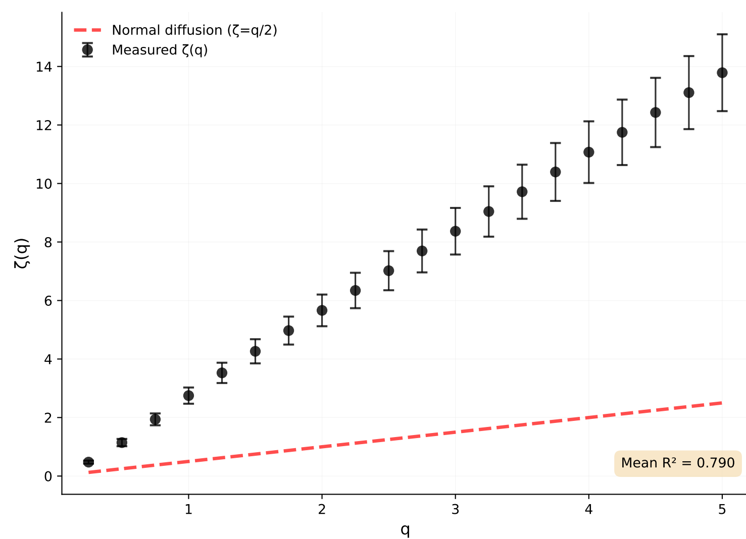
Coda
