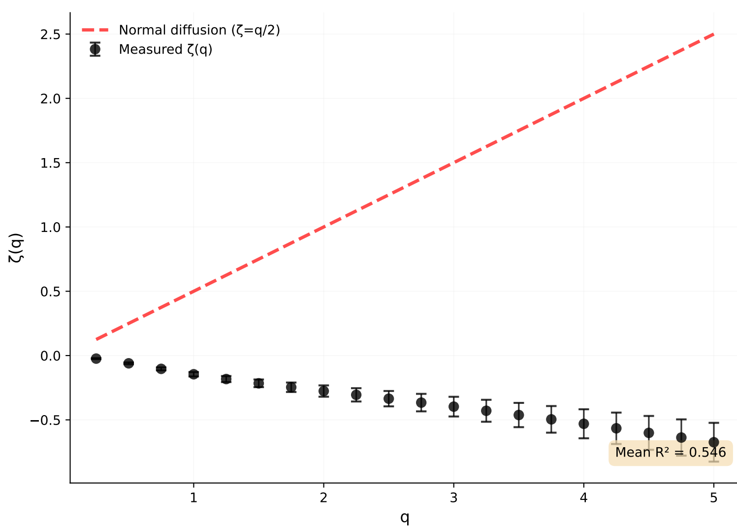
Coda
