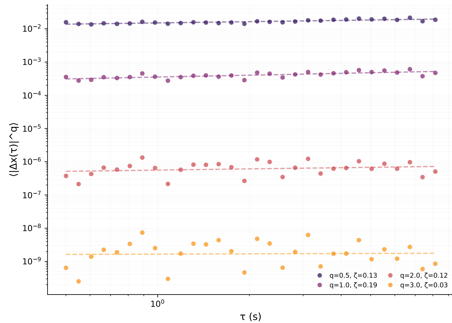
S-wave
