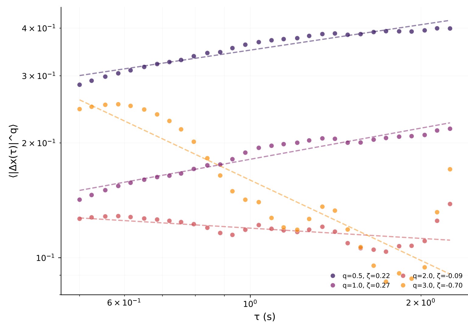
Coda
