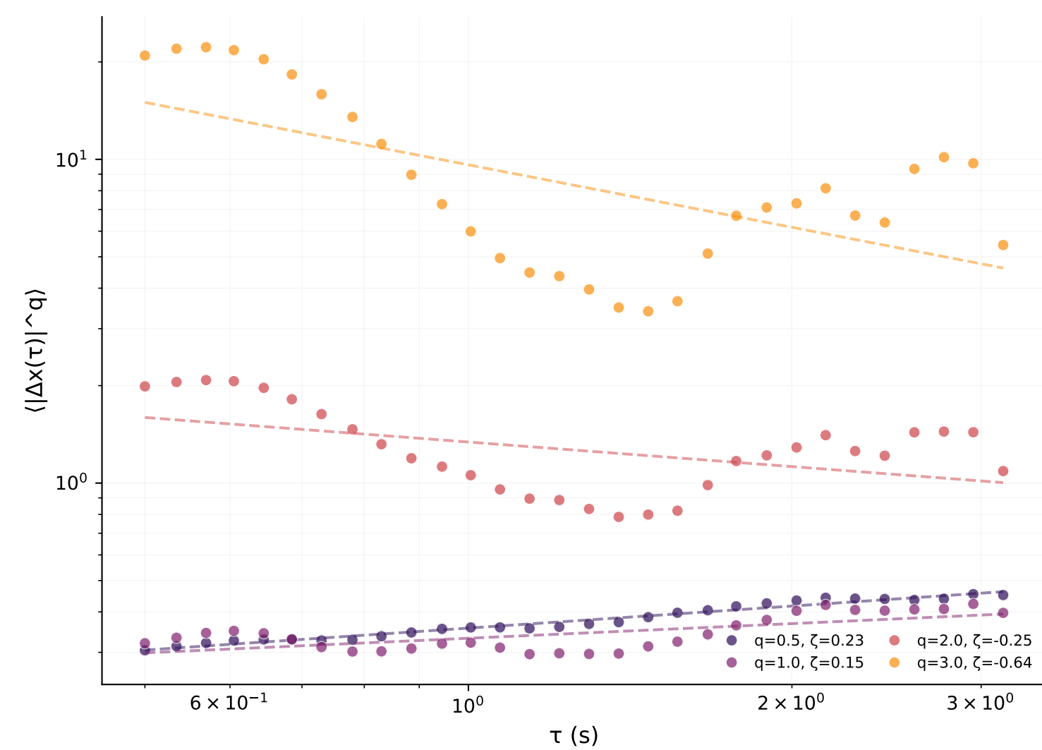
S-wave
