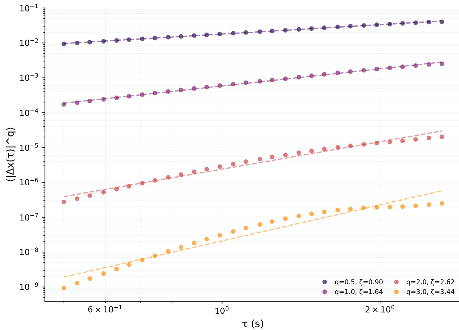
Pre-event (noise)
