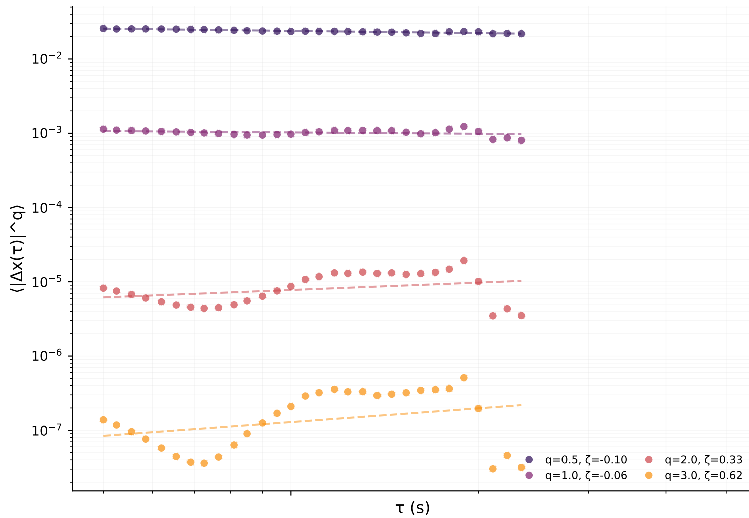
S-wave
