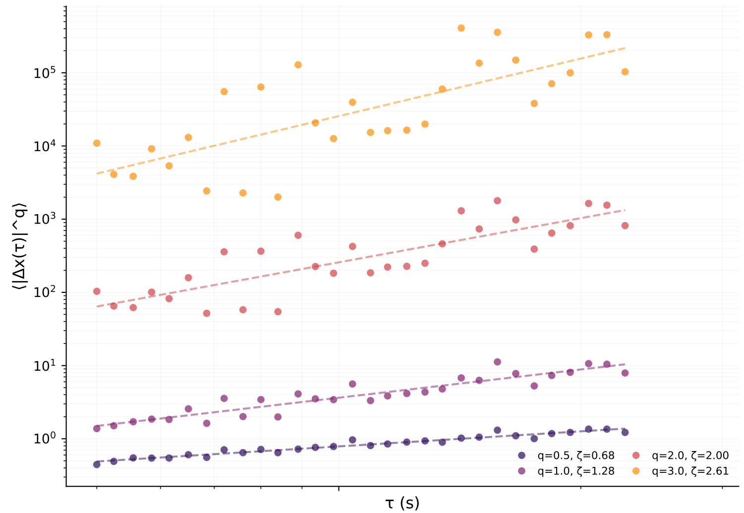
Coda
