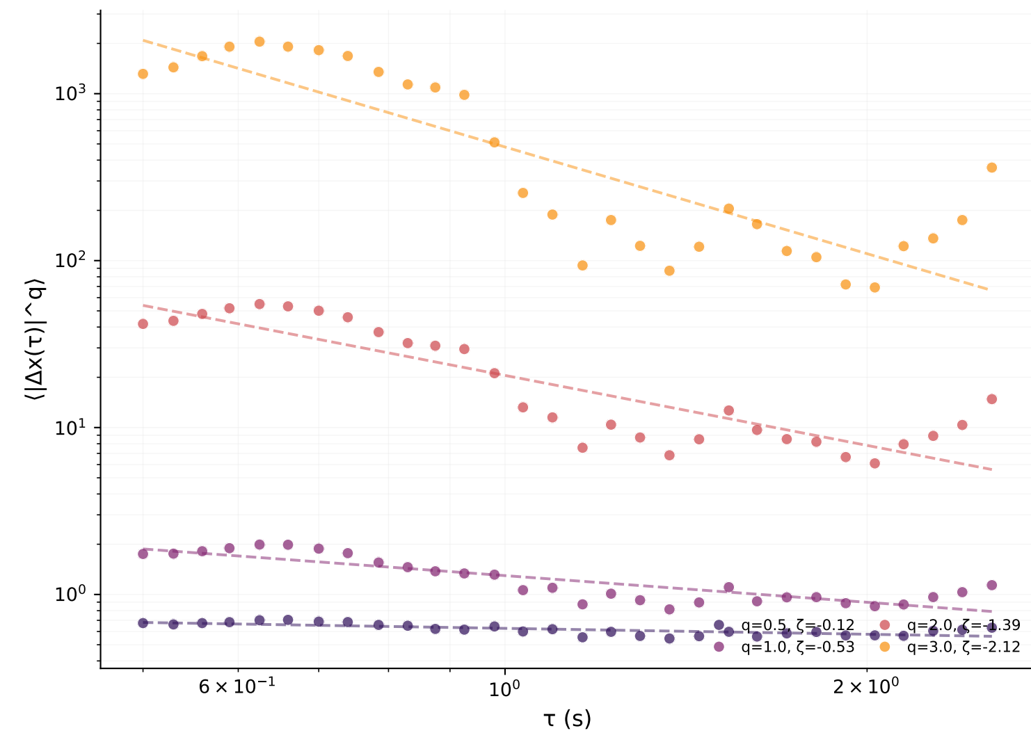
S-wave
