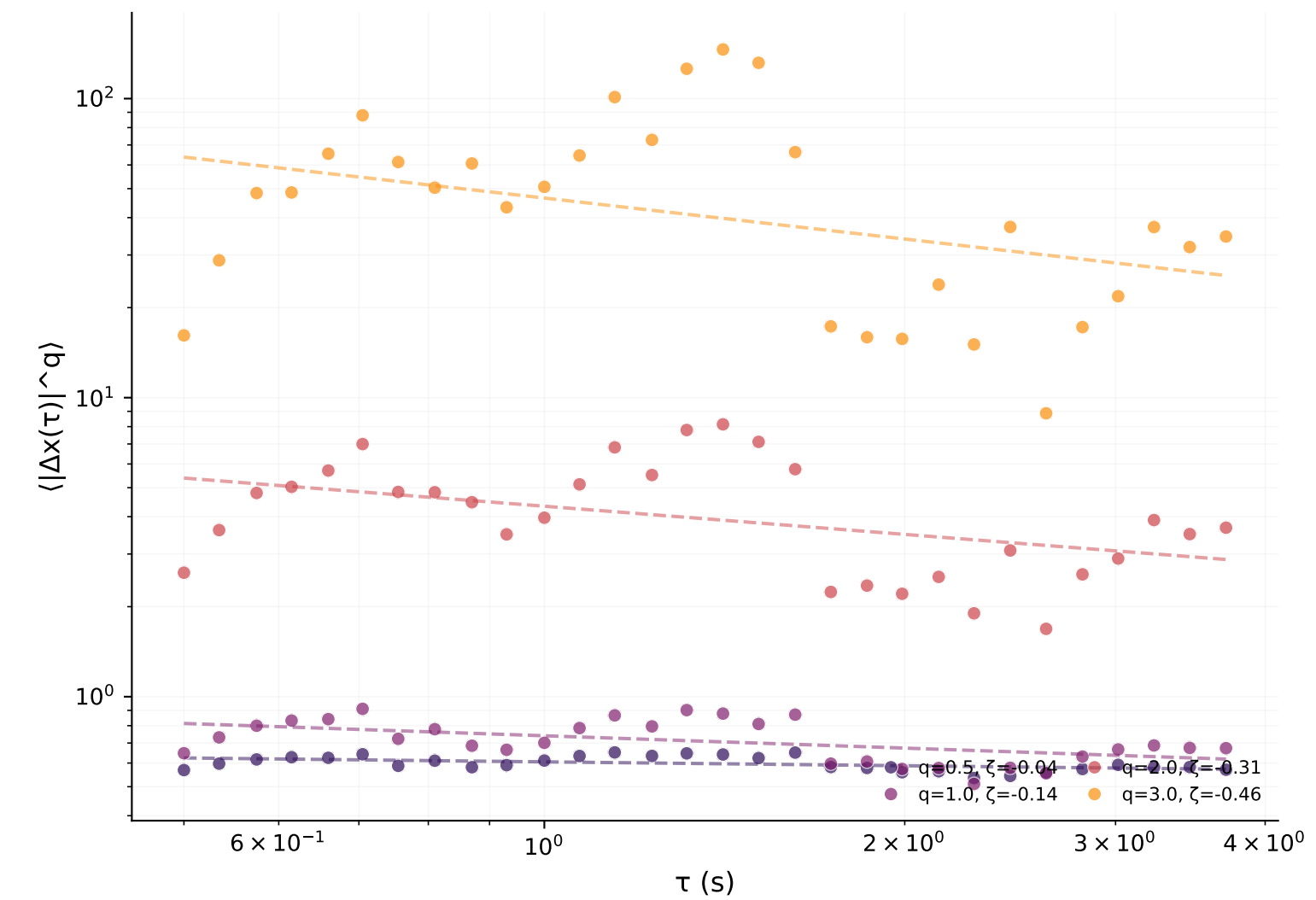
Coda
