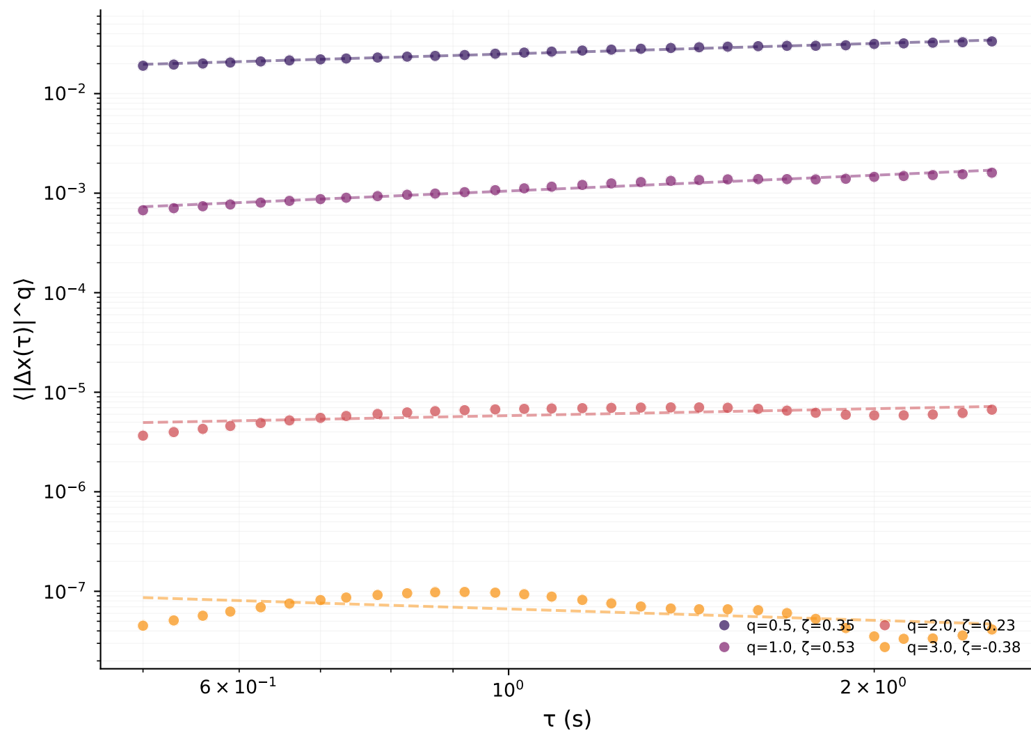
S-wave
