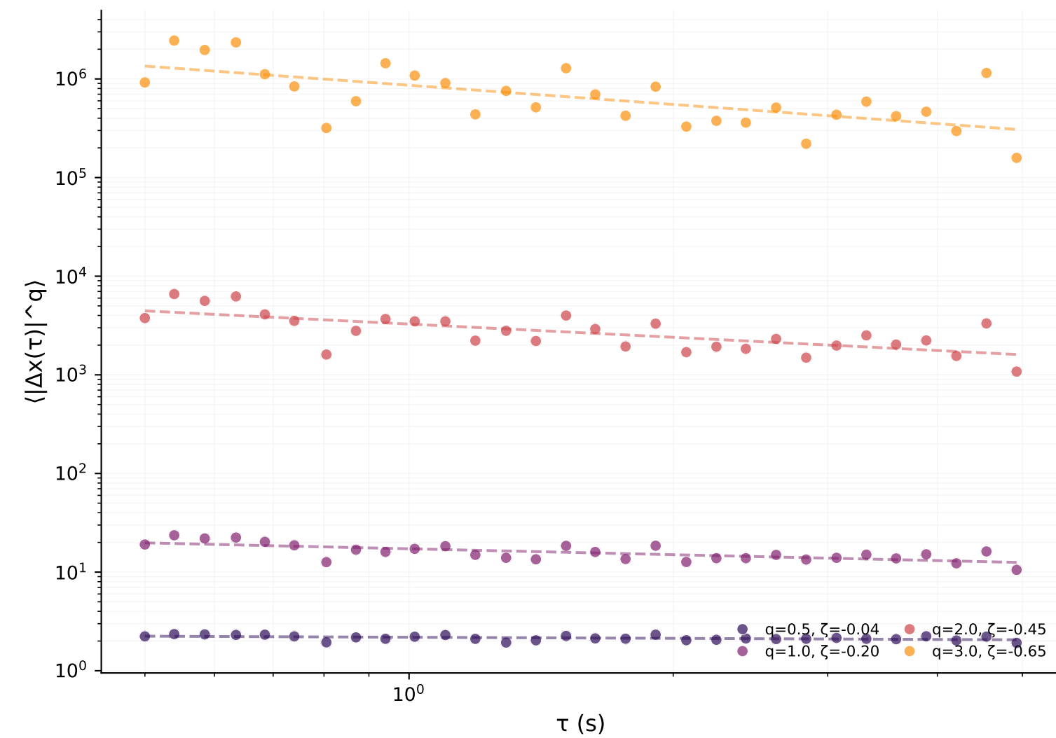
S-wave
