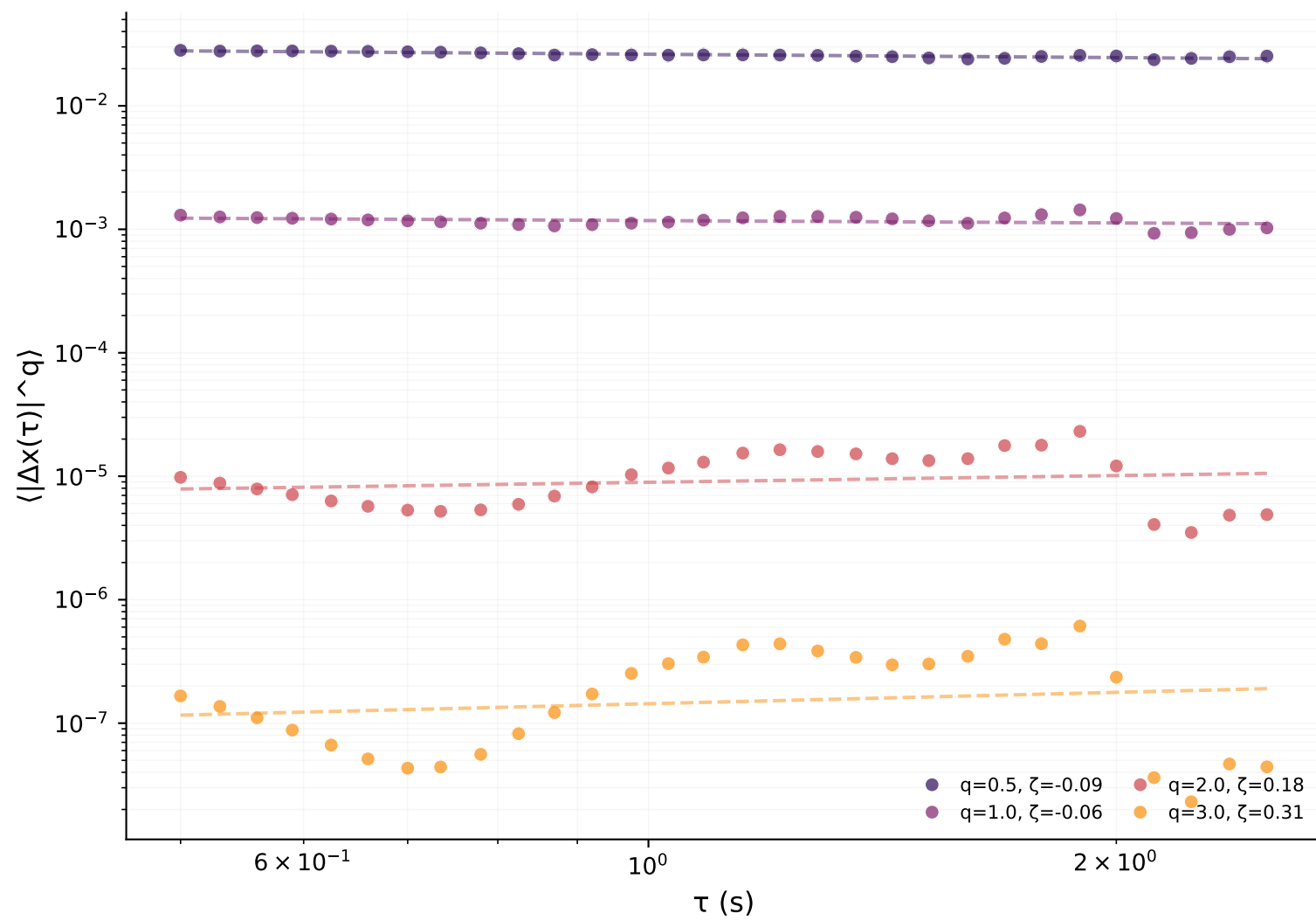
S-wave
