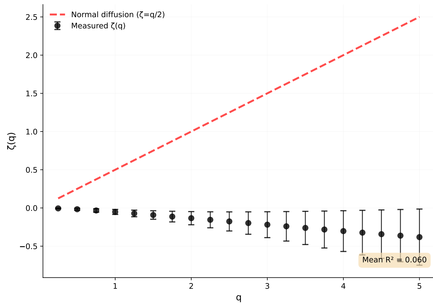
Coda
