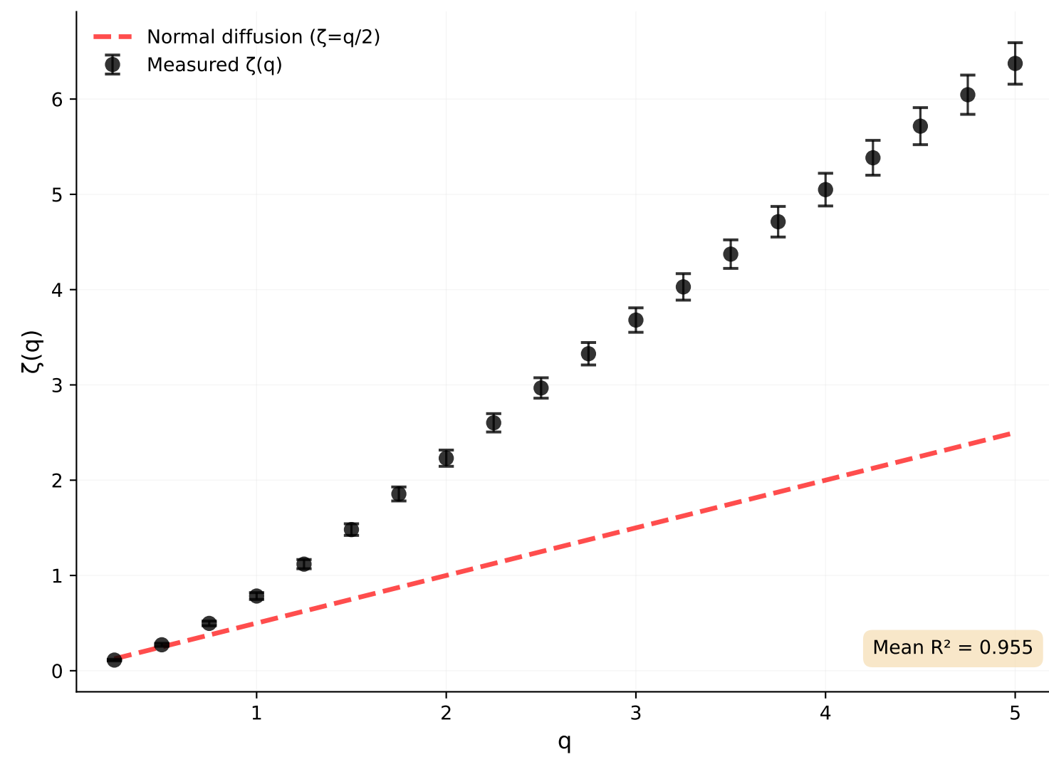
Coda
