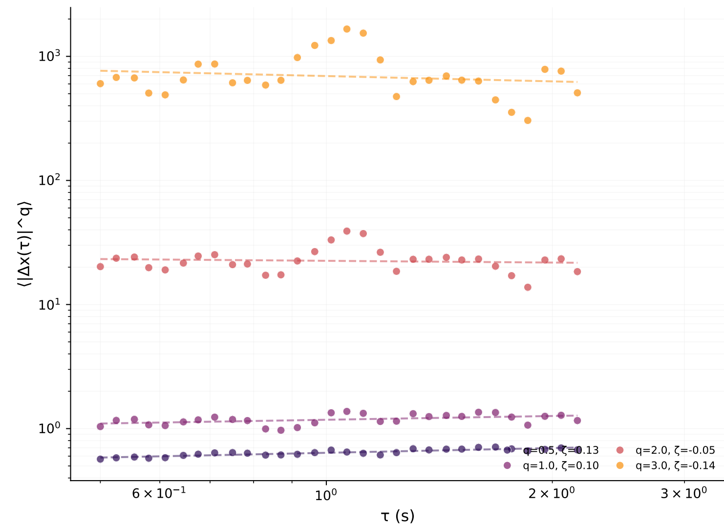
S-wave
