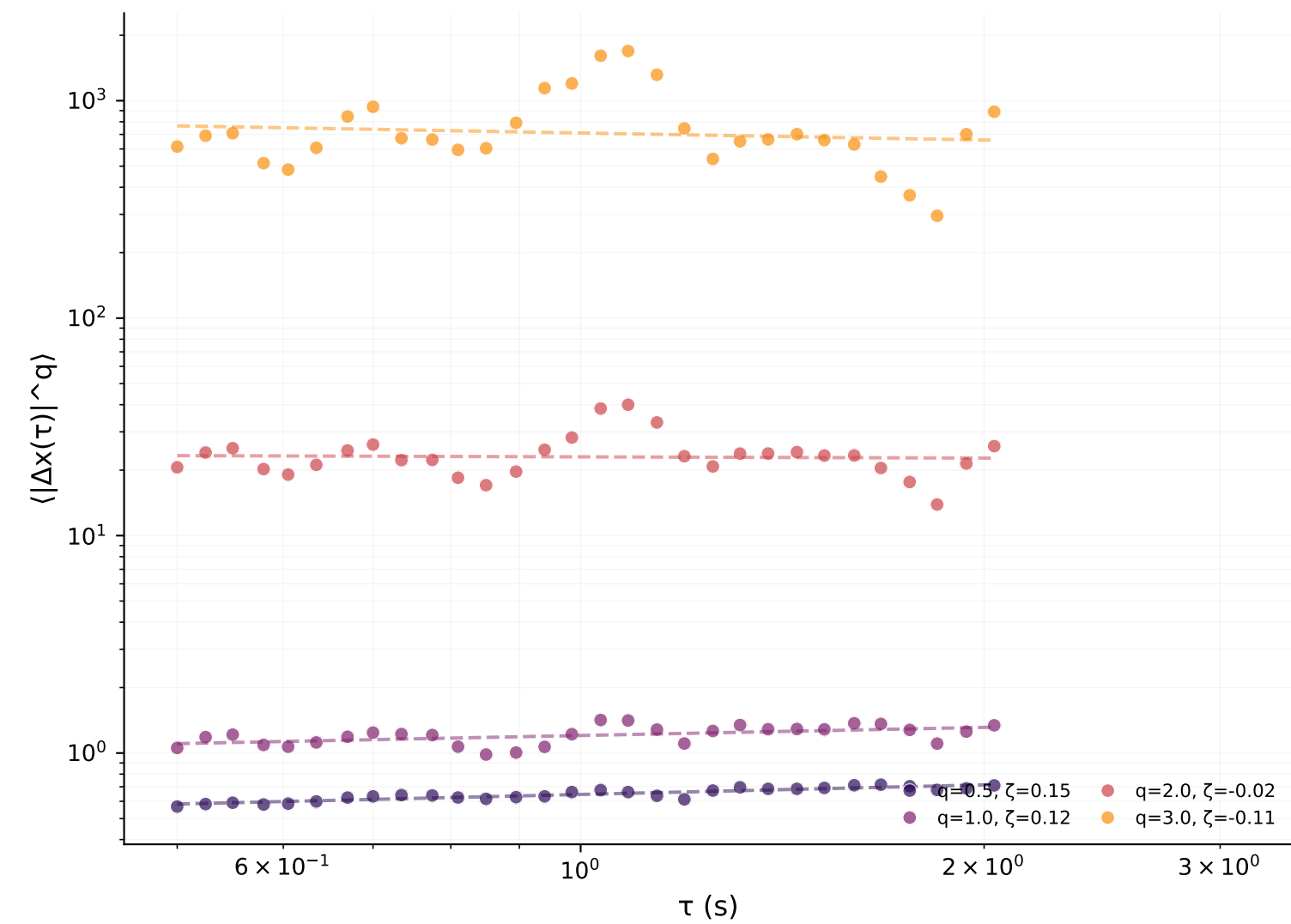
S-wave
