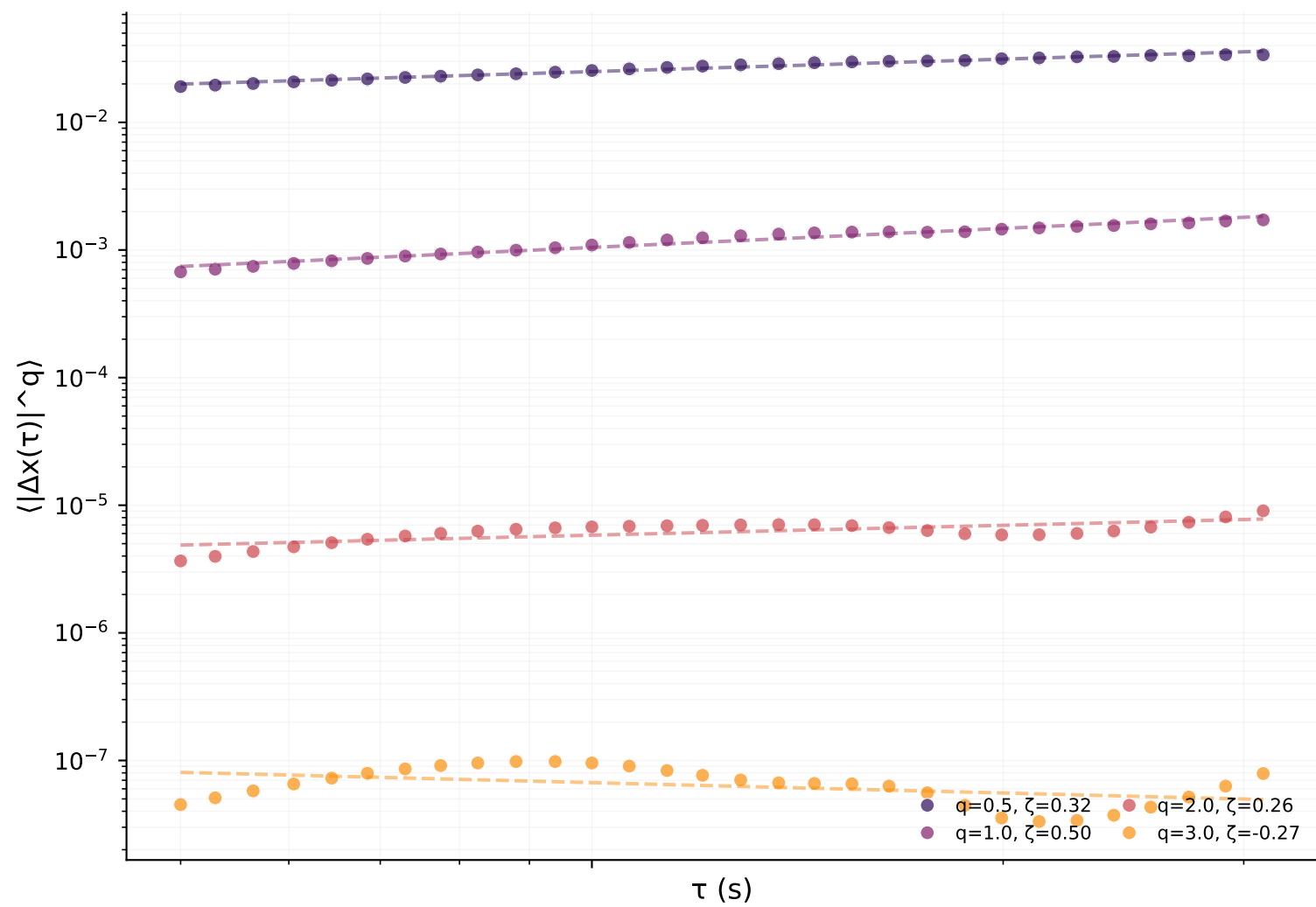
S-wave
