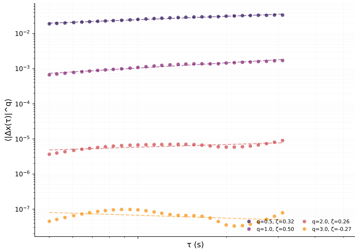
S-wave
