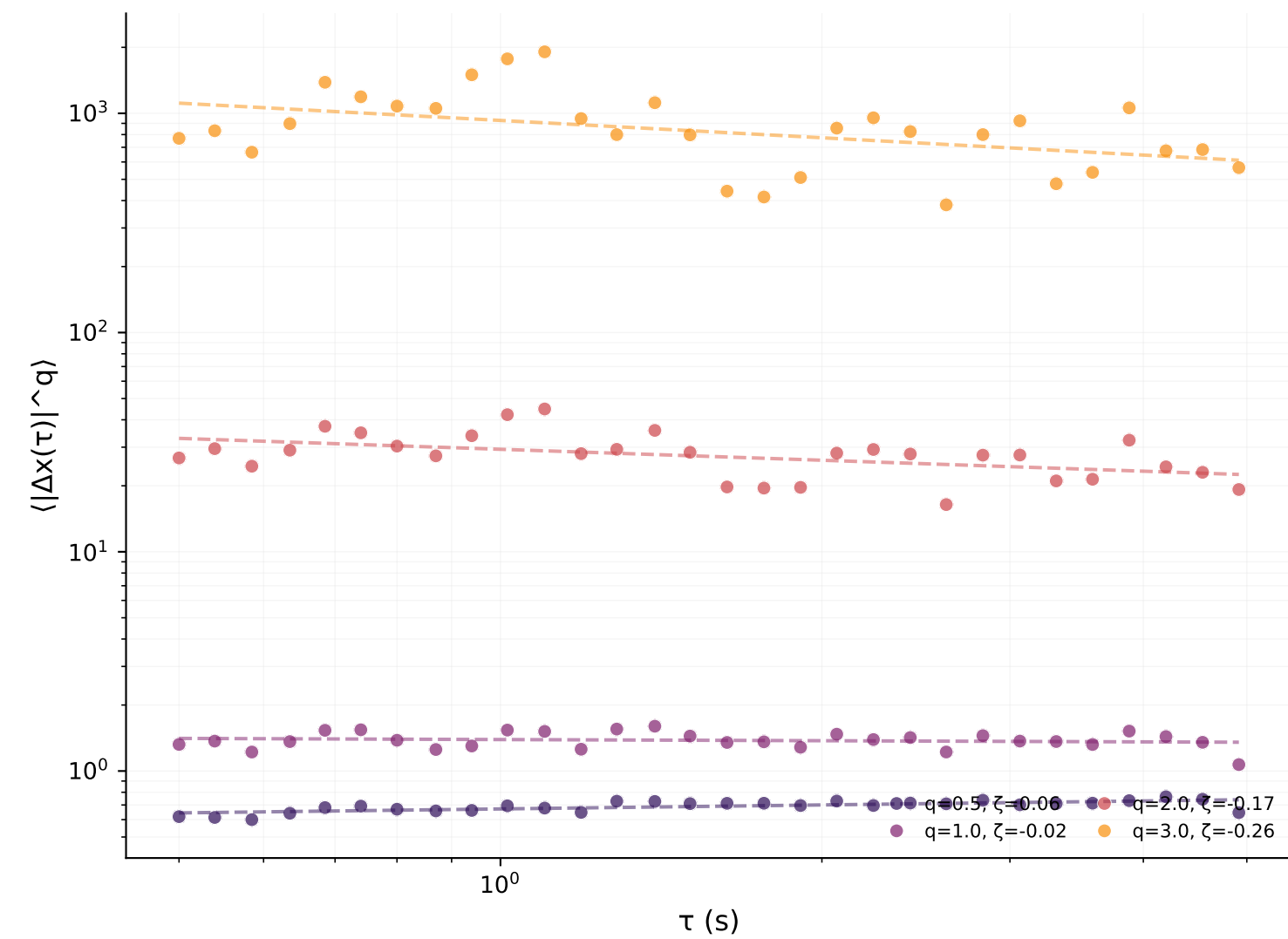
S-wave
