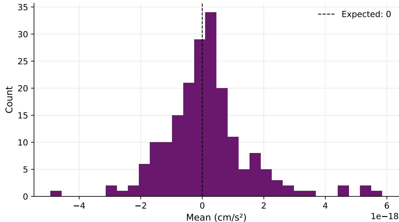
Baseline correction — SANL HNE
