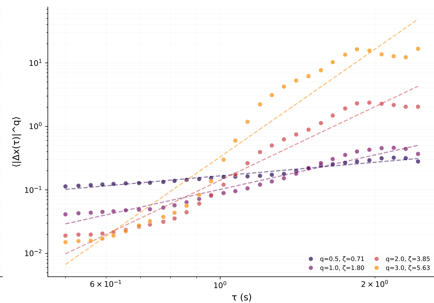
P-wave
