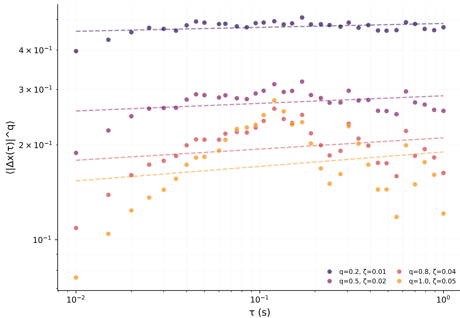
S-wave
