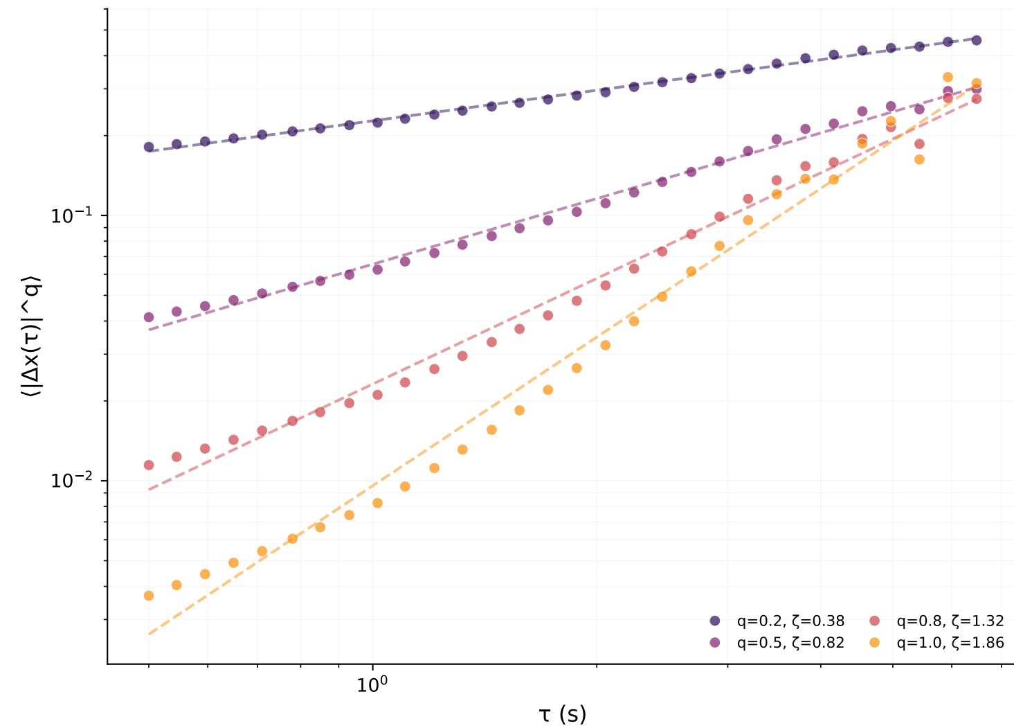
Coda
