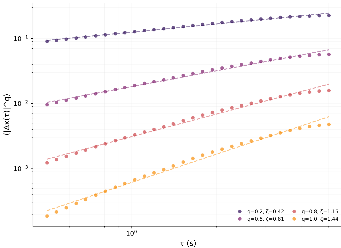
S-wave
