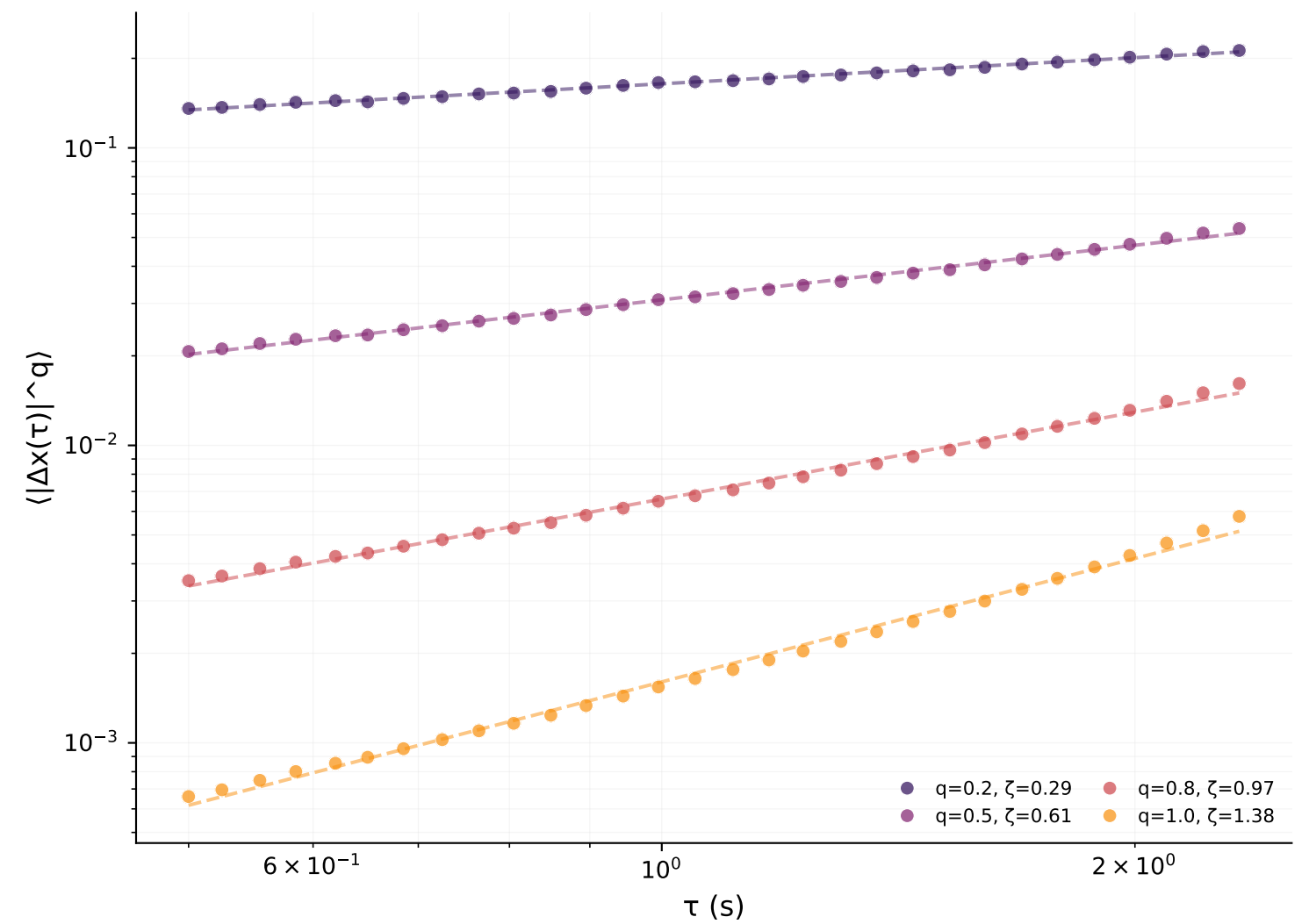
Coda
