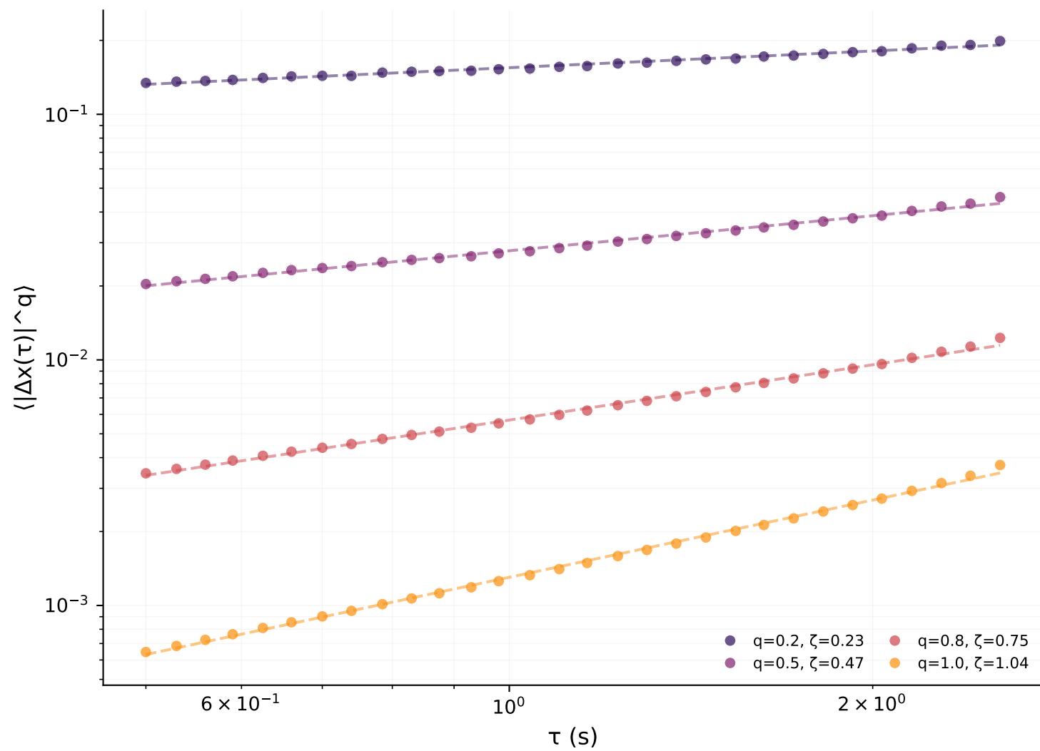
S-wave
