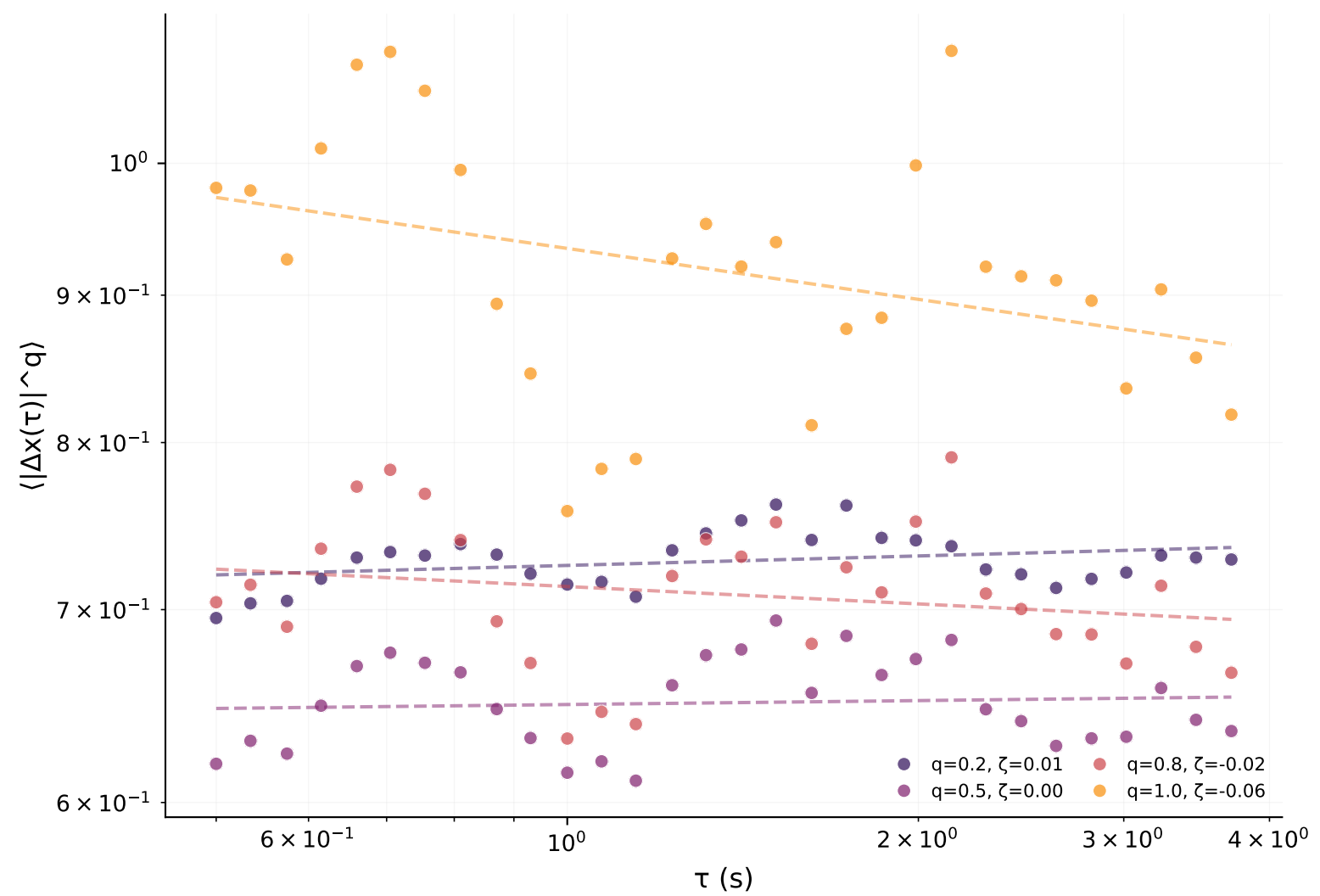
Coda
