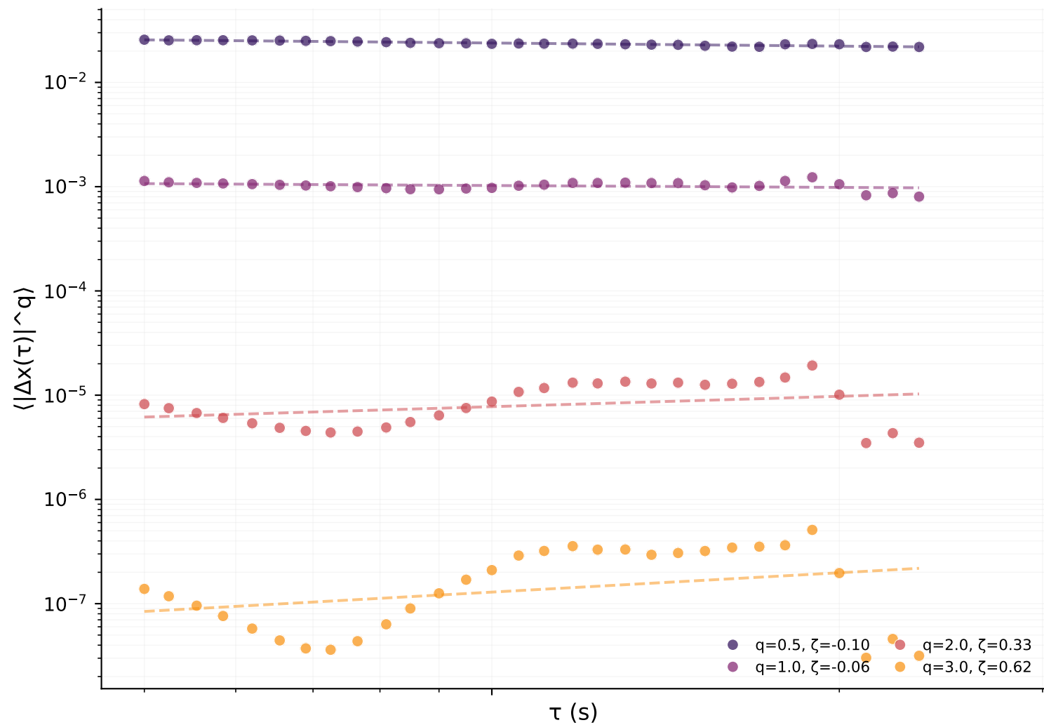
S-wave
