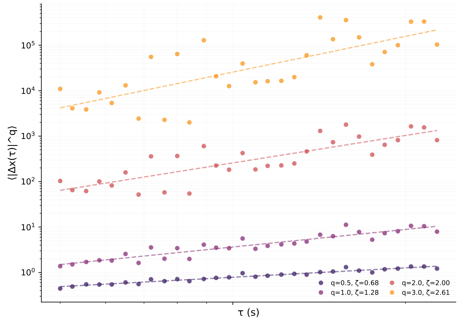
Coda
