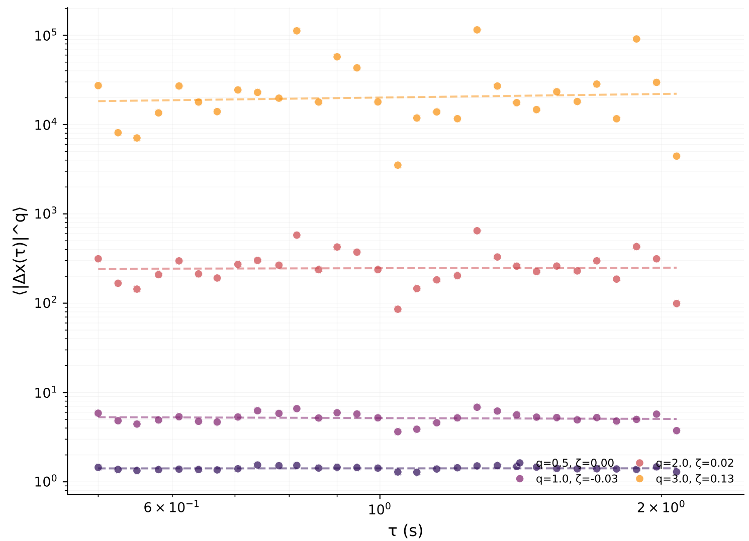
Coda
