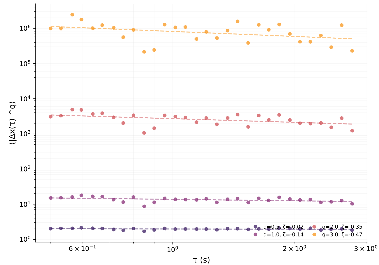
S-wave
