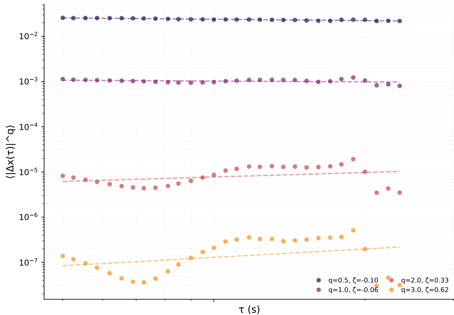
S-wave
