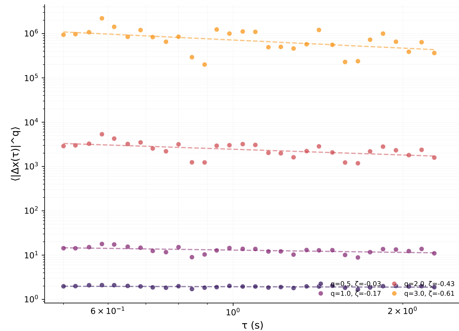
S-wave
