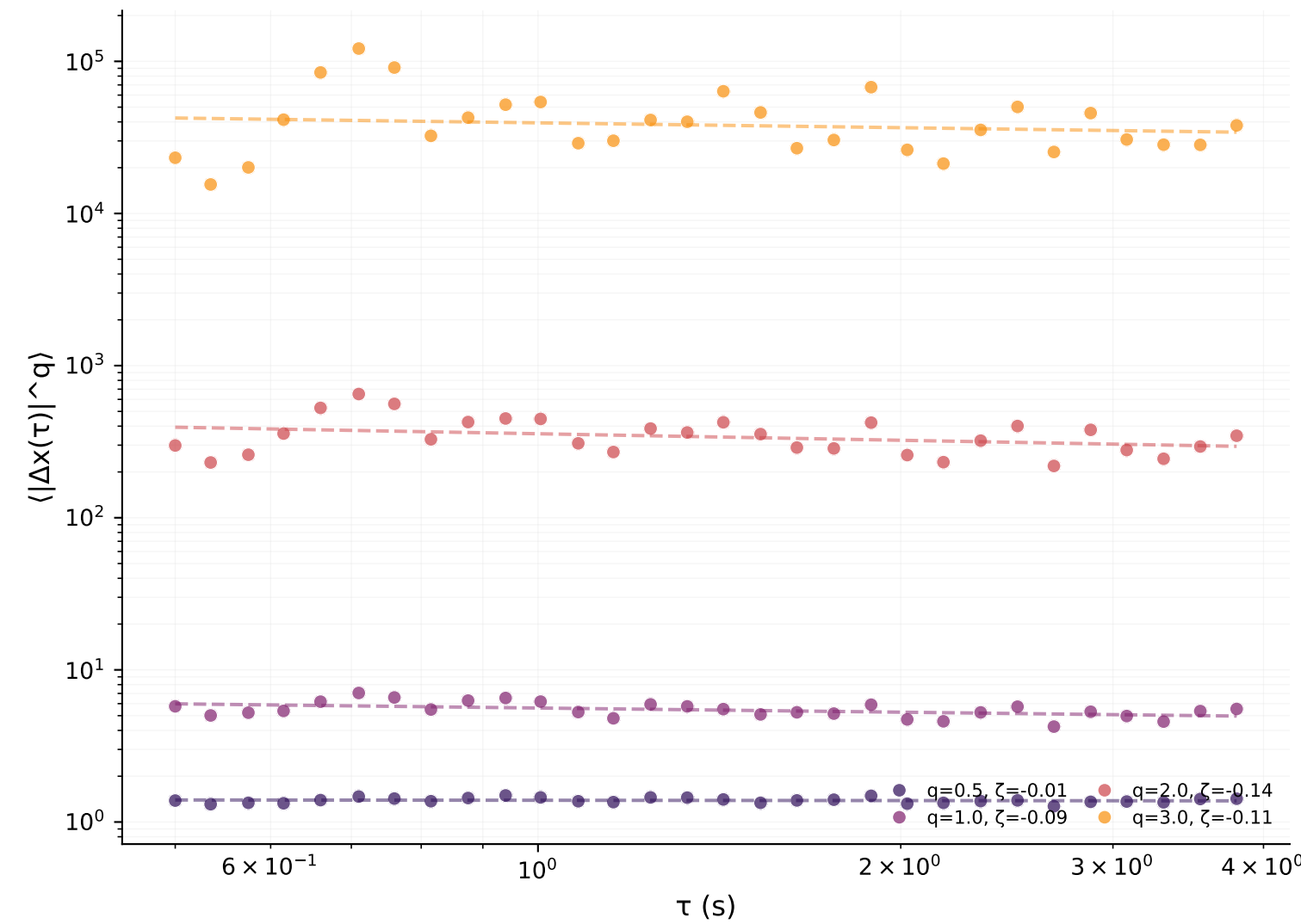
Coda
