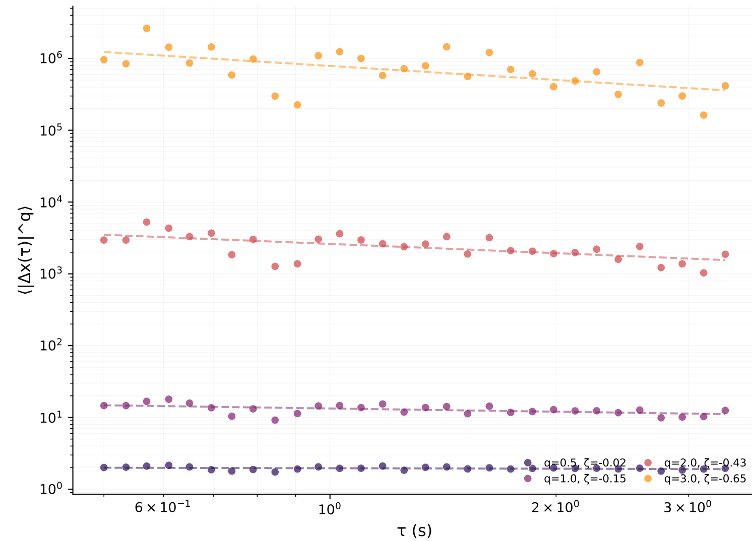
S-wave
