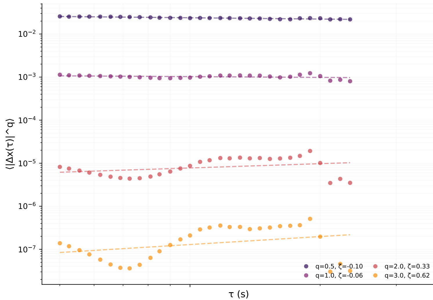
S-wave
