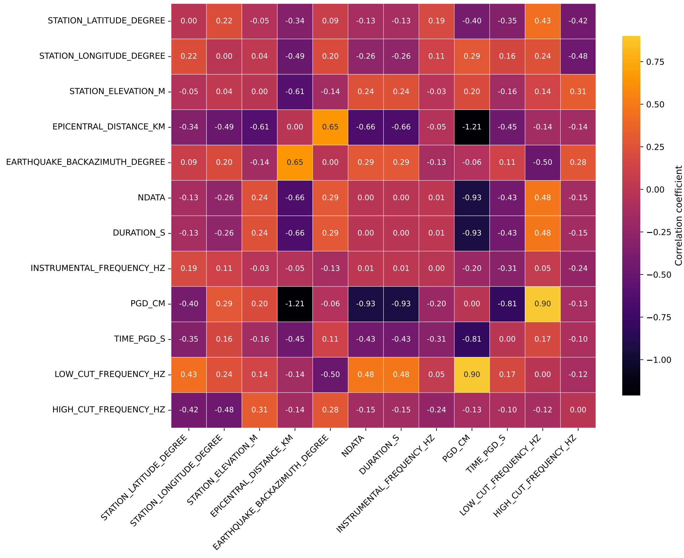
Correlation difference: Near vs Far
