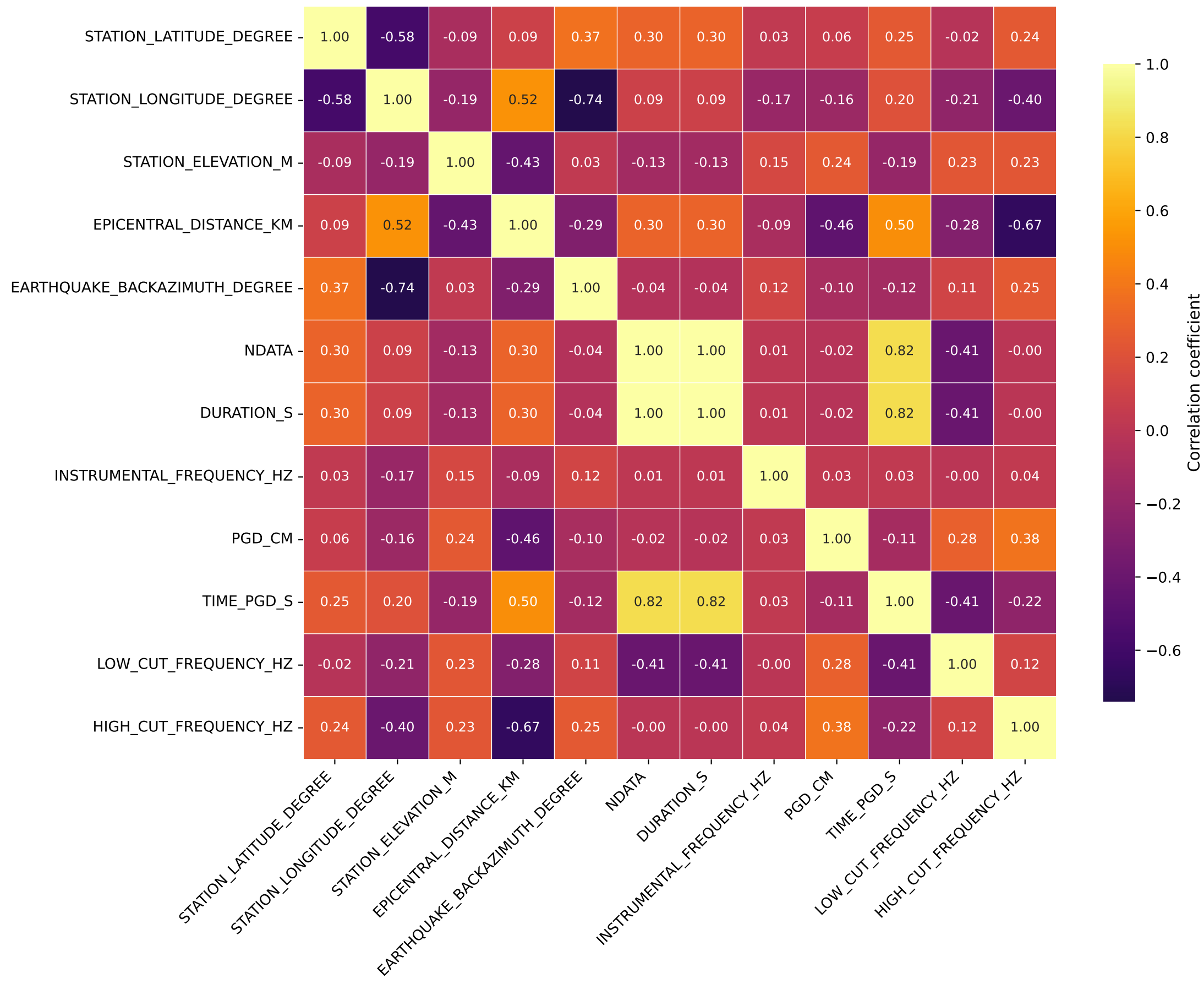
Correlation matrix of numerical variables
