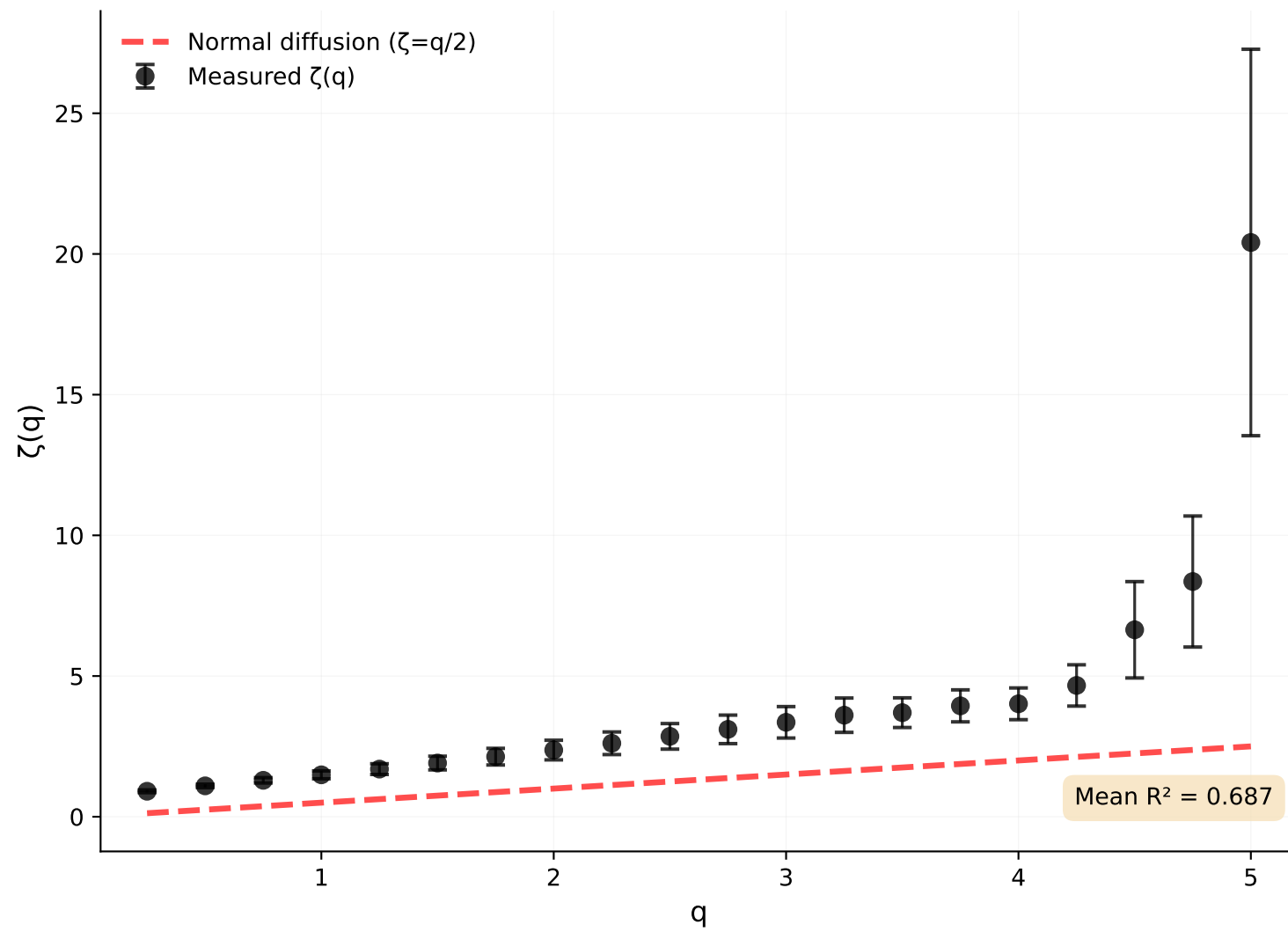
S-wave
