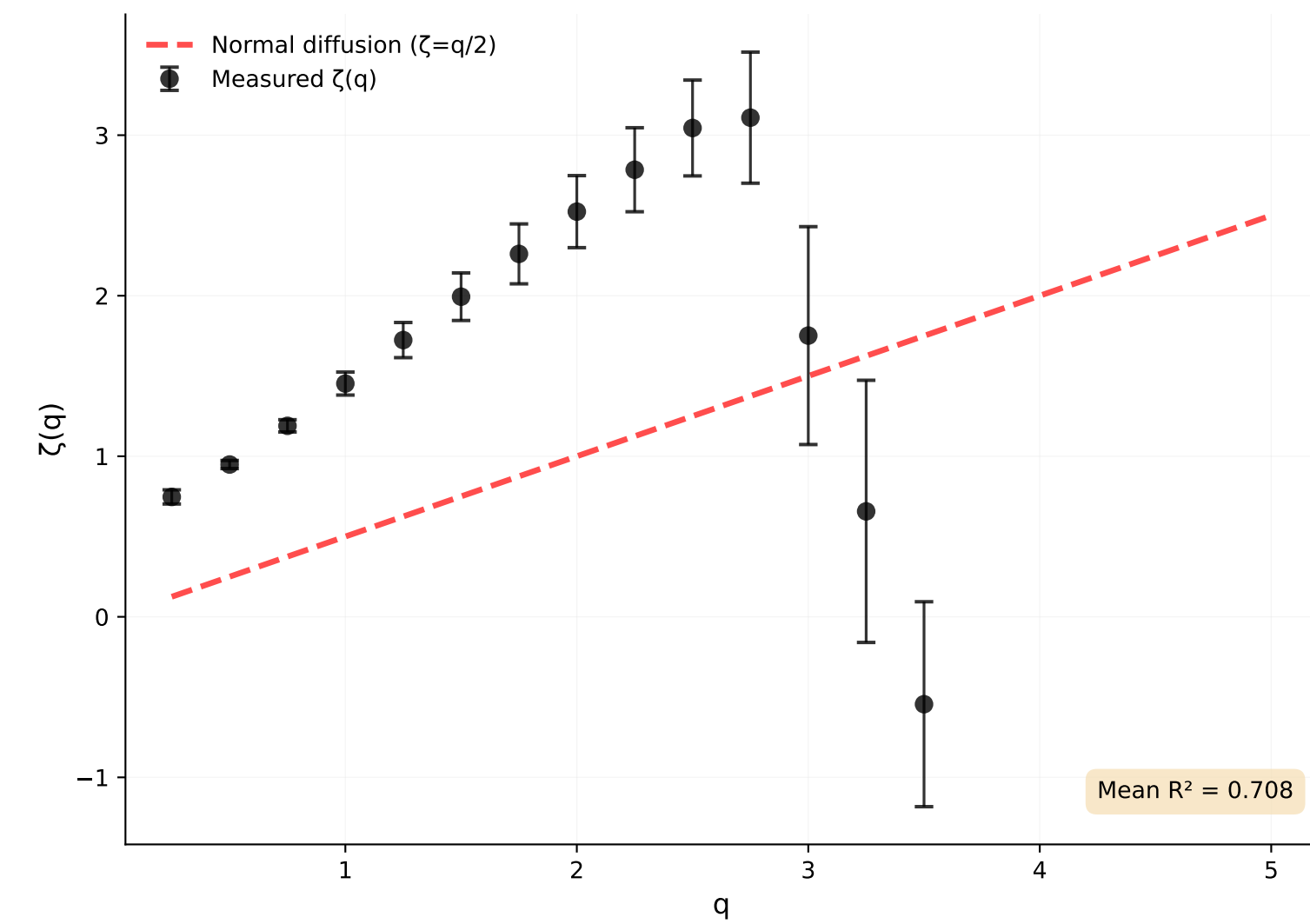
S-wave
