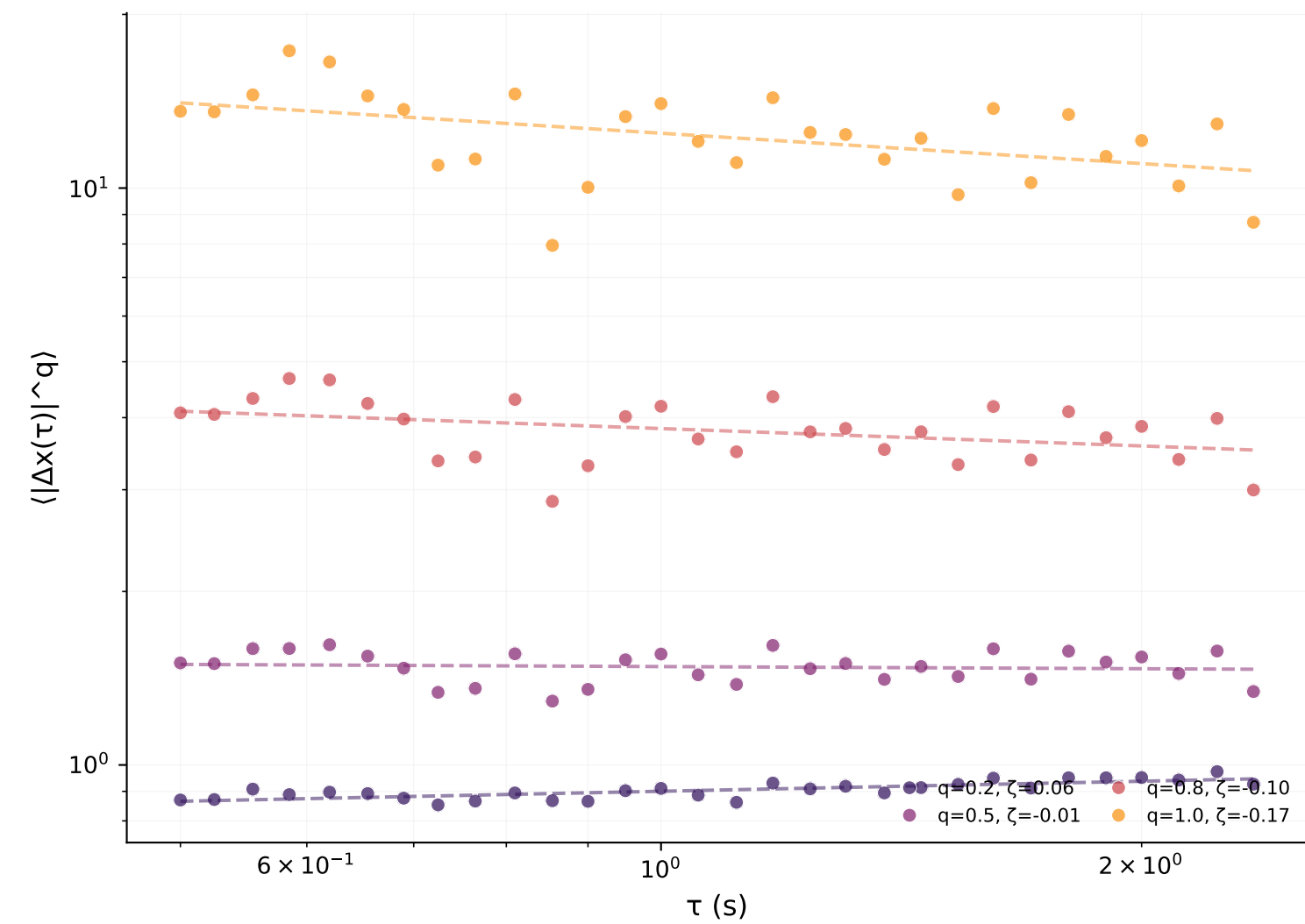
S-wave
