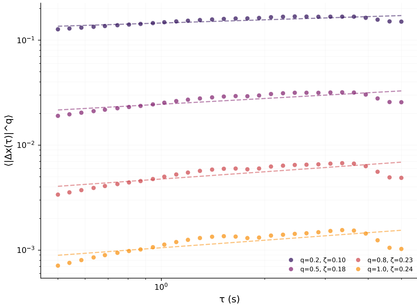
S-wave
