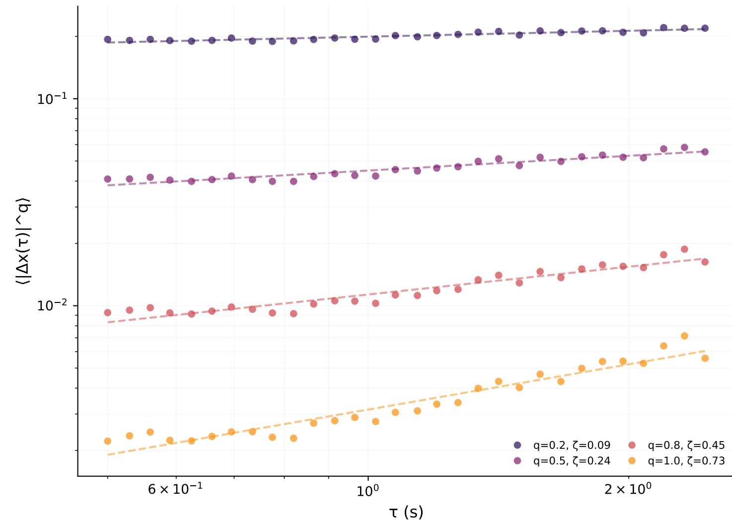
Coda
