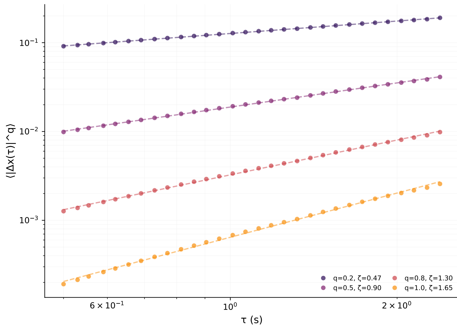
S-wave
