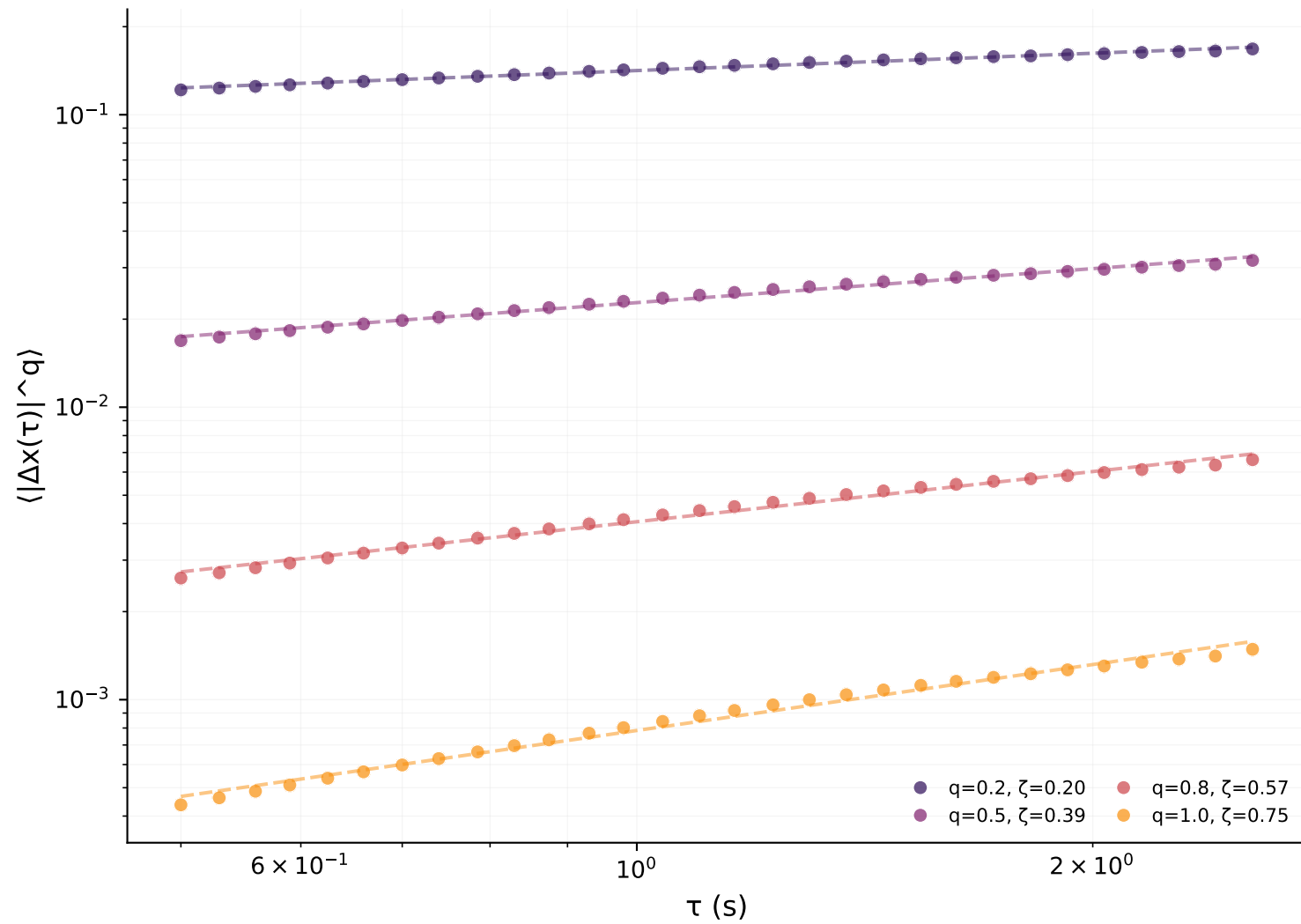
S-wave
