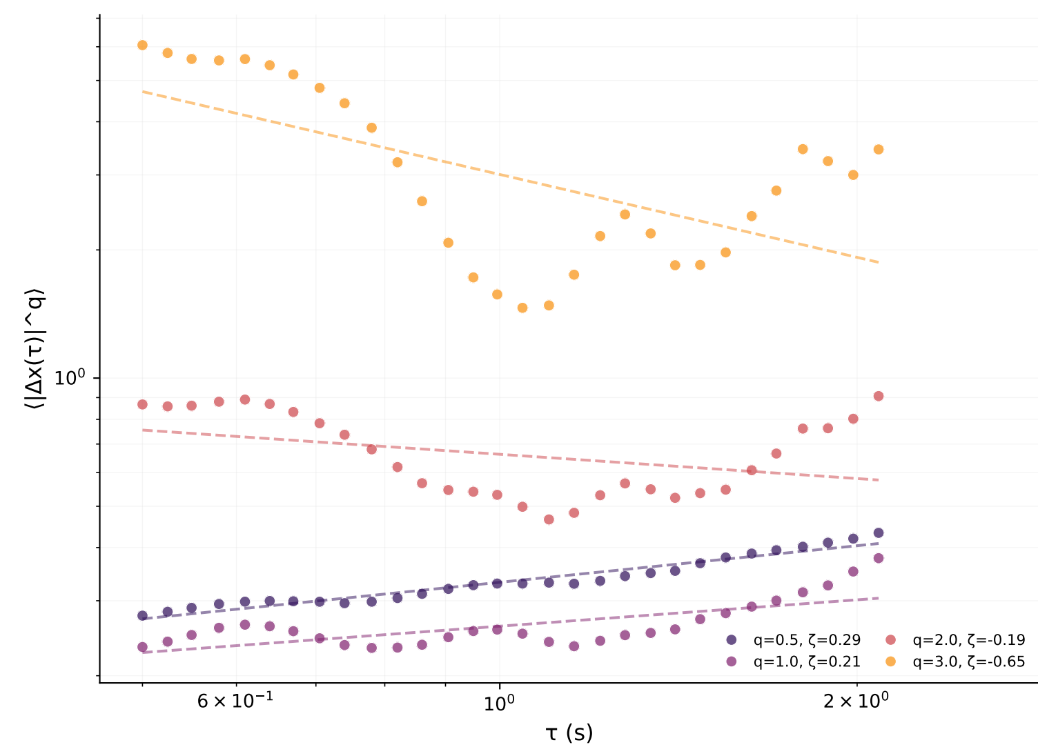
S-wave
