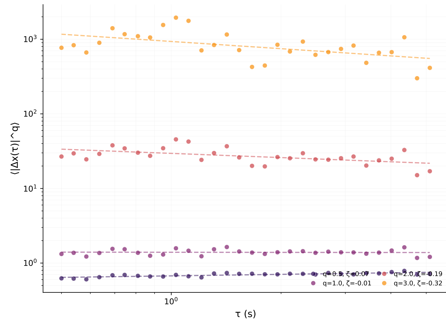
S-wave
