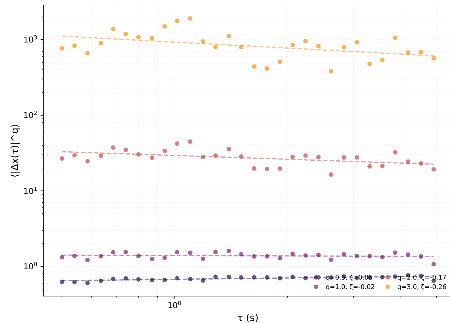
S-wave
