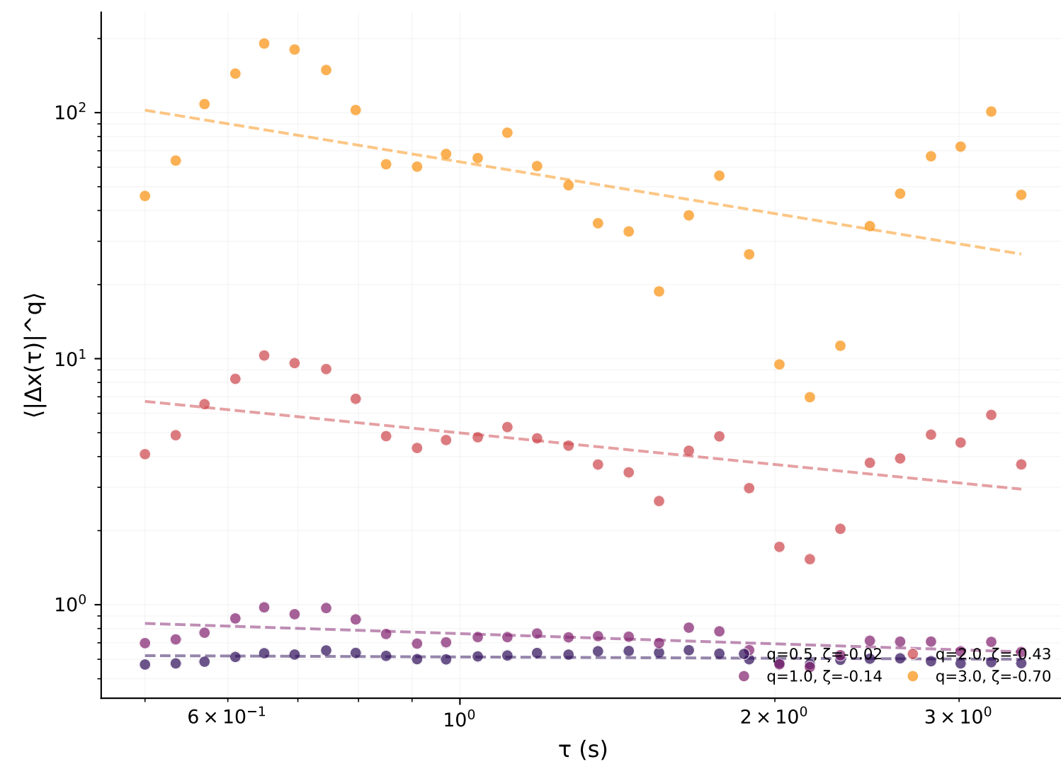
Coda
