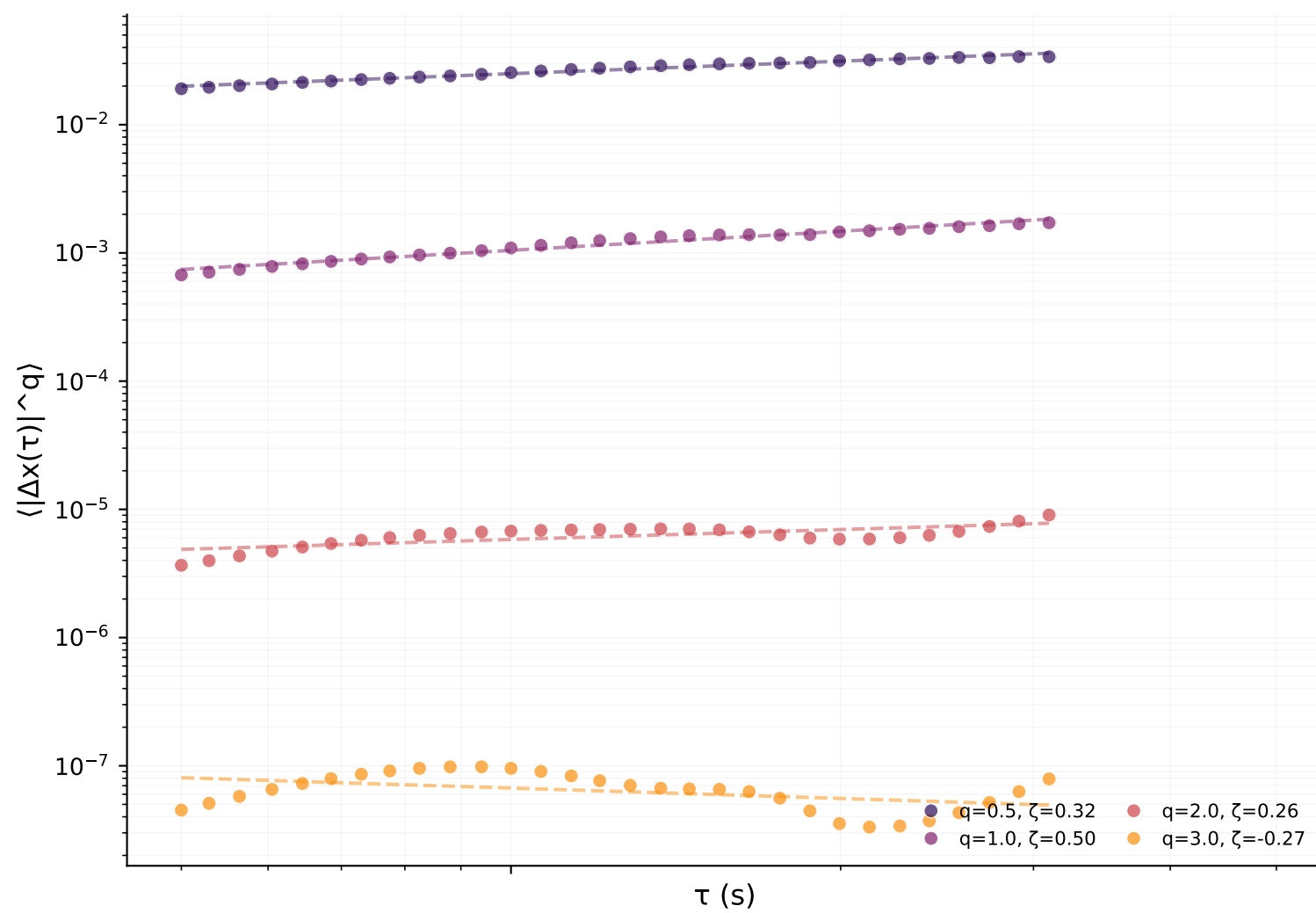
S-wave
