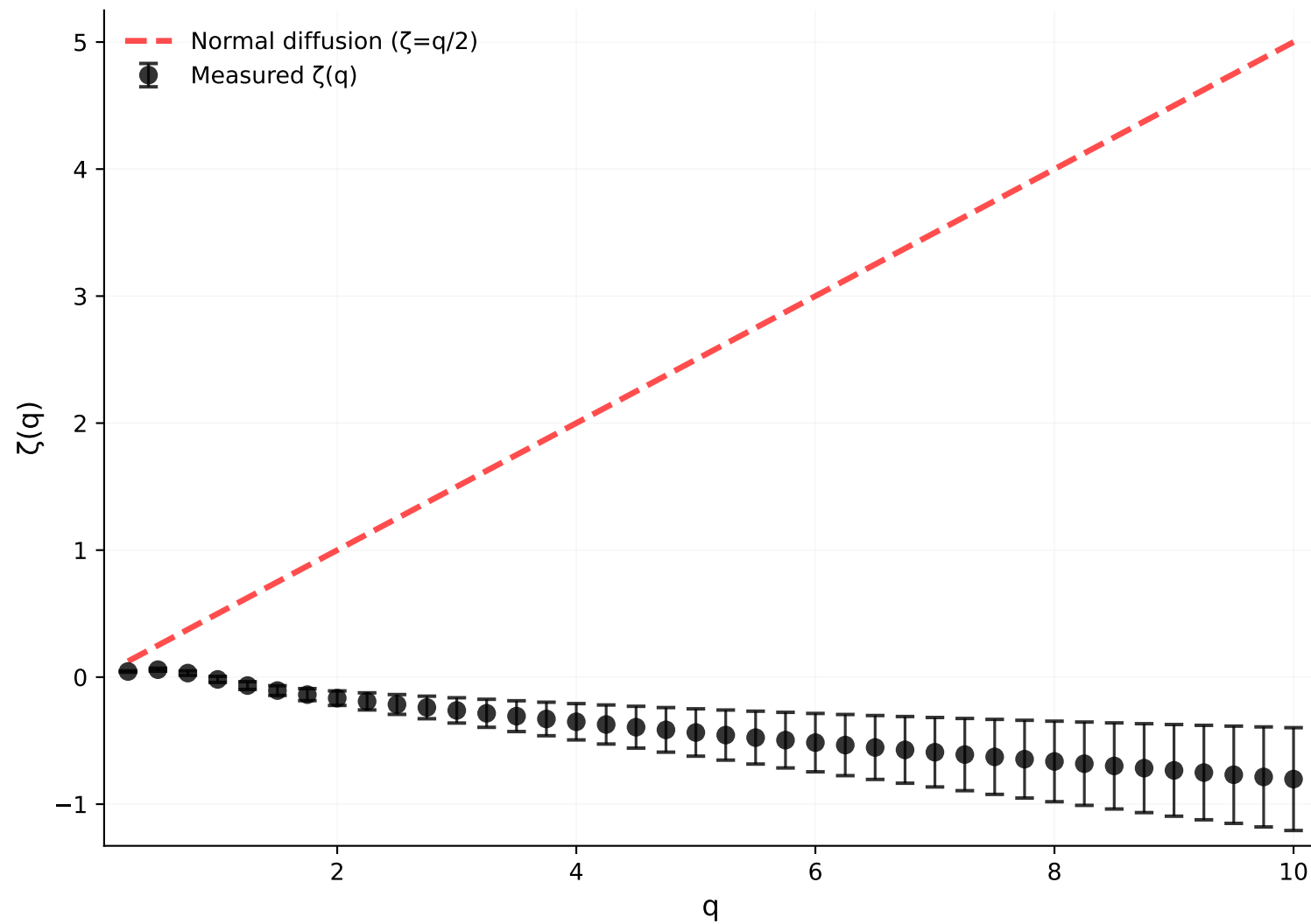
S-wave
