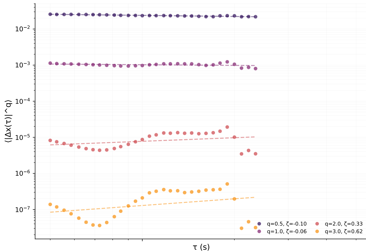
S-wave
