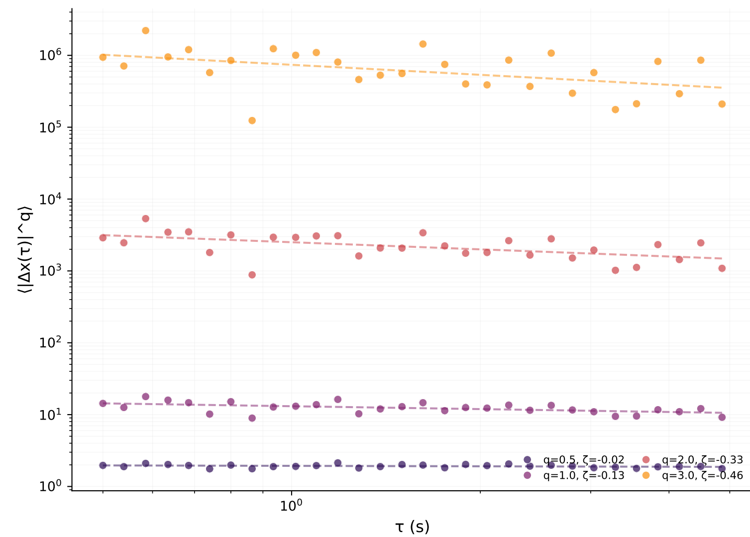
S-wave
