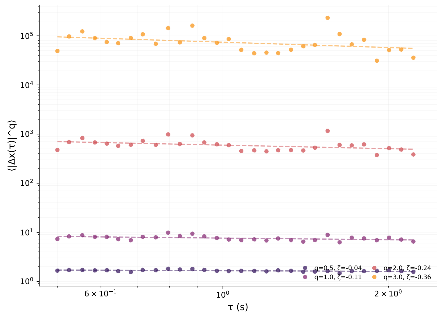
Coda
