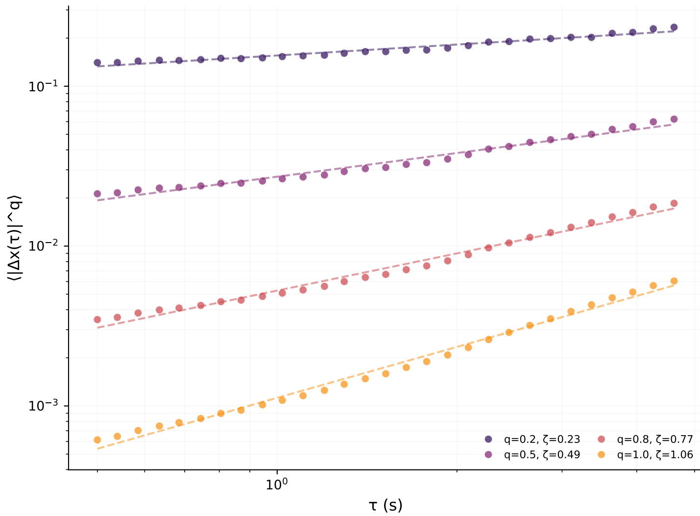
S-wave
