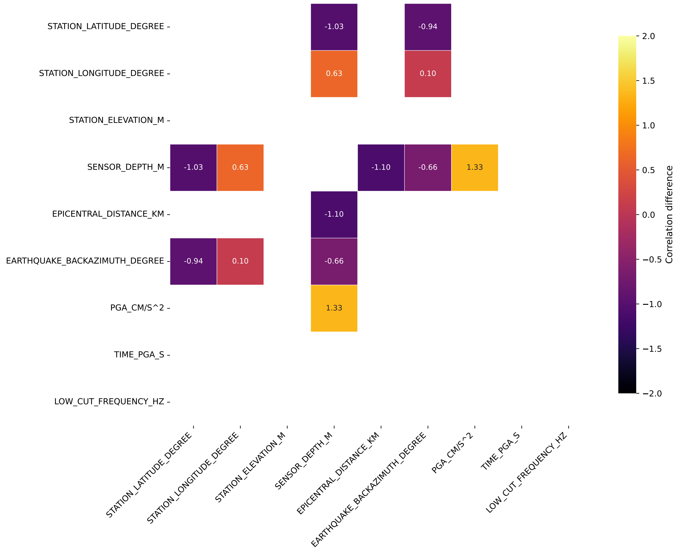
Significant correlation differences (p&lt;0.05): Near vs Far
