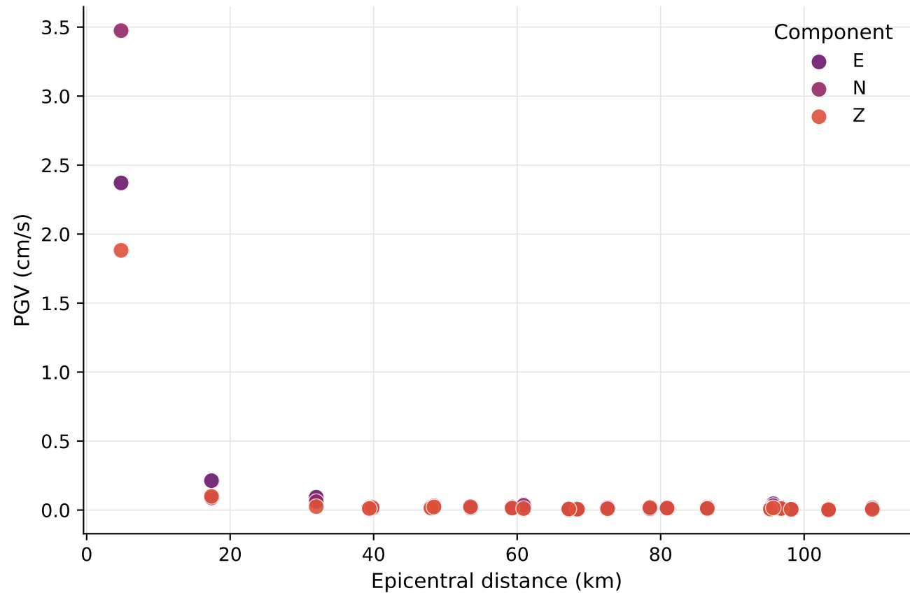
PGV vs epicentral distance by component
