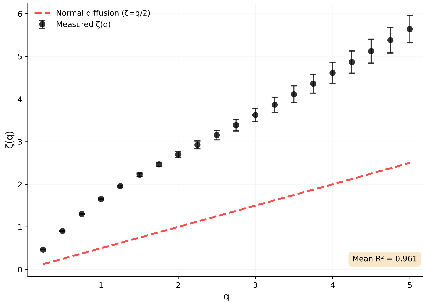
S-wave
