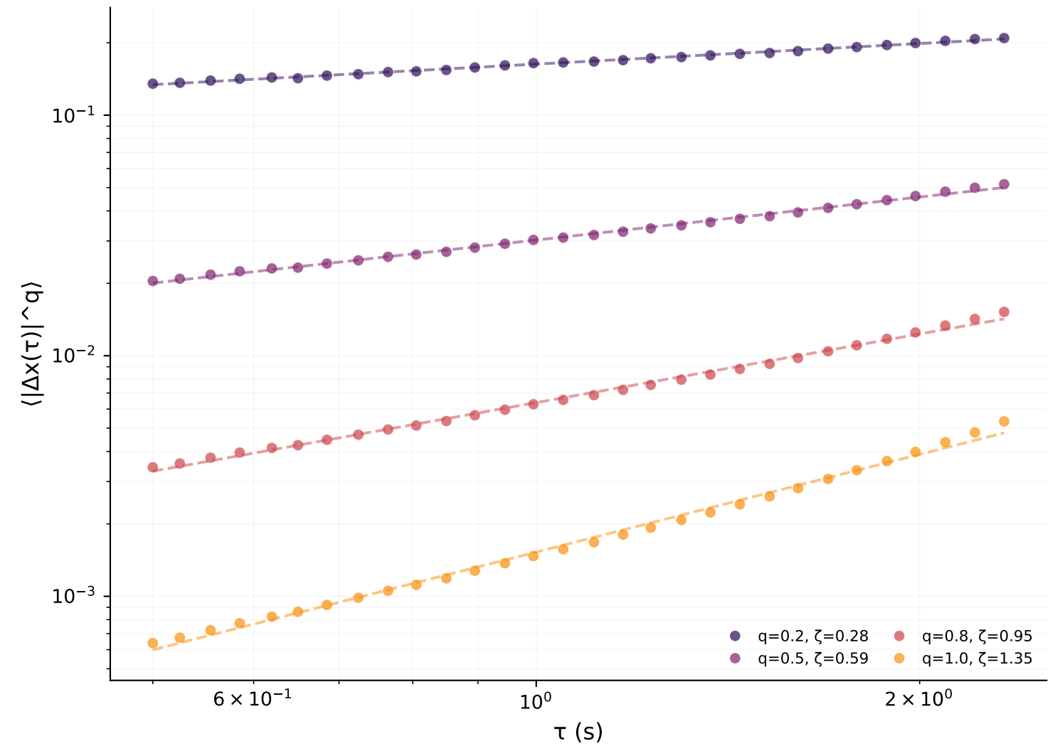
Coda
