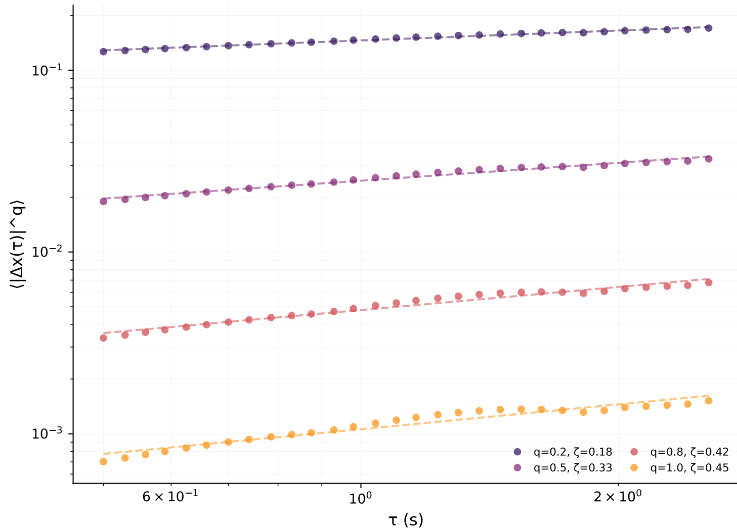
S-wave
