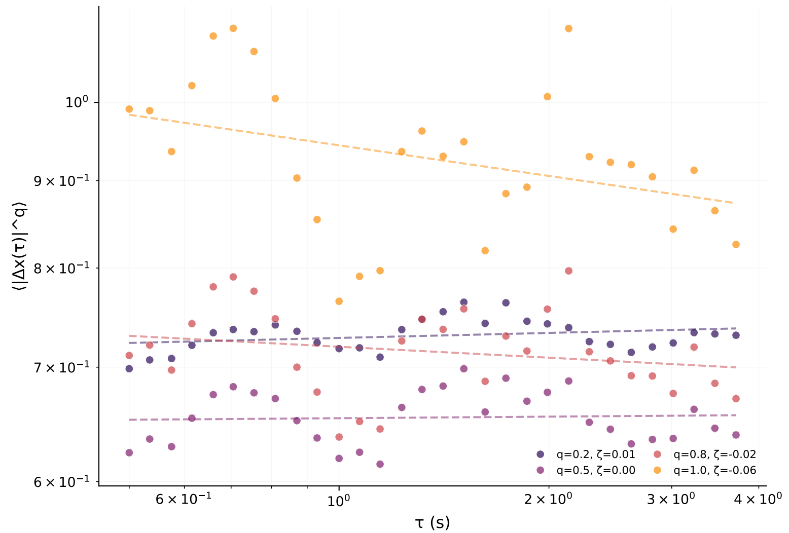
Coda
