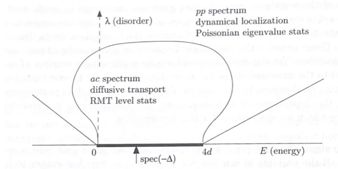
Figure 1: For small disorder localisation is not expected
