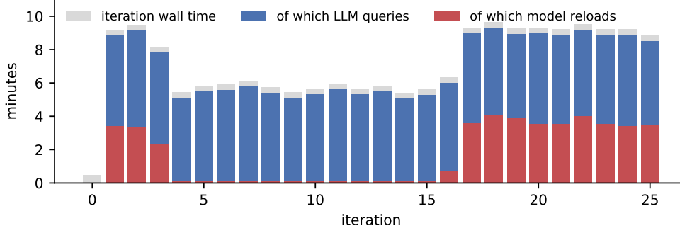
Figure 3: Iteration wall time. Grey: whole iteration; blue: the ten LLM queries; red: the part spent reloading the model after another user’s job.
