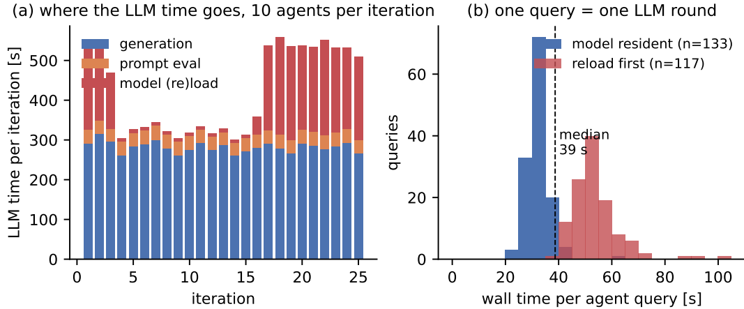
Figure 2: LLM time. (a) Per iteration, split into generation, prompt evaluation and model loading. (b) Wall time per query.
