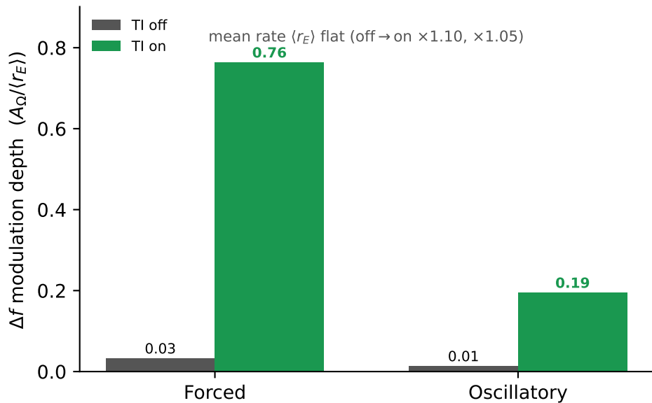
(b) TI imposes \Delta f -locked timing, not rate
