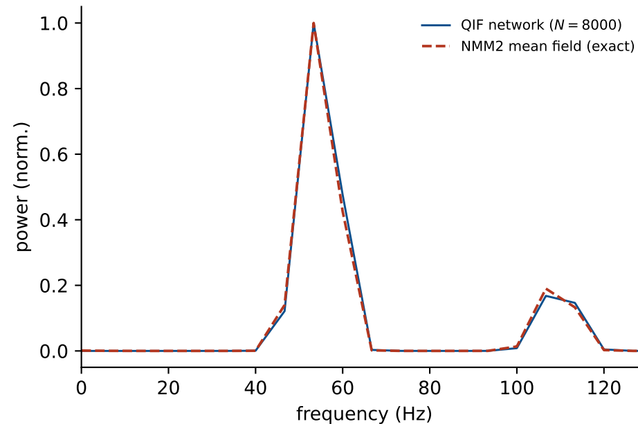
(a) QIF \rightarrow NMM2: matched autonomous gamma ( \langle r_E \rangle : 0.053 QIF vs 0.052 mean field)
