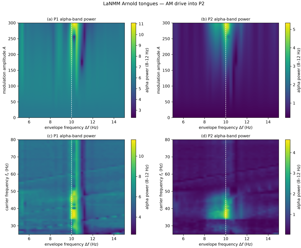
Figure 8: LaNMM Arnold tongues: AM input to the superficial P_2 (gamma) loop. (a,b) Alpha-band power of P_1 and P_2 vs. modulation amplitude A and beat frequency \Delta f (carrier 40 Hz): a tongue of elevated power around the P_1 alpha ( \sim 10 Hz, dashed line) that widens with A . (c,d) Alpha power vs. carrier frequency and \Delta f at A = 250 : P_1 demodulation requires both a carrier \approx 40 Hz ( P_2 gamma) and \Delta f \approx 10 Hz ( P_1 alpha)—a double resonance.
