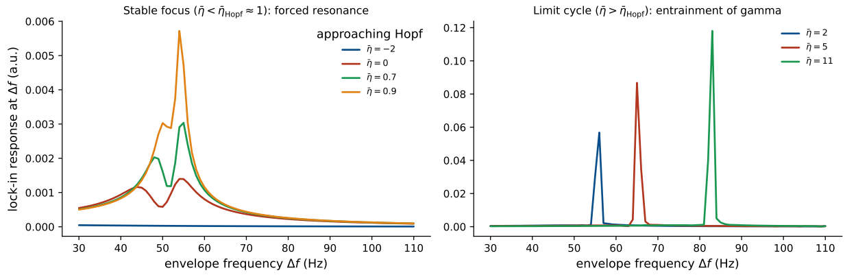
Figure 9: NMM2 PING gamma resonance (exact mean field). Lock-in response of the excitatory rate r_E at the envelope frequency \Delta f under an AM field (carrier 300 Hz). Left (stable focus, \bar{\eta} < \bar{\eta}_{\text{Hopf}} \approx 1 ): forced resonance at the gamma frequency ( f_0 \approx 55 Hz), growing as the Hopf is approached ( 1/\gamma gain), with the resonant frequency rising with \bar{\eta} . Right (limit cycle, \bar{\eta} > \bar{\eta}_{\text{Hopf}} ): entrainment of the autonomous gamma. The input carries no power at \Delta f ; the response is synthesized by the exact quadratic v^2 nonlinearity.
