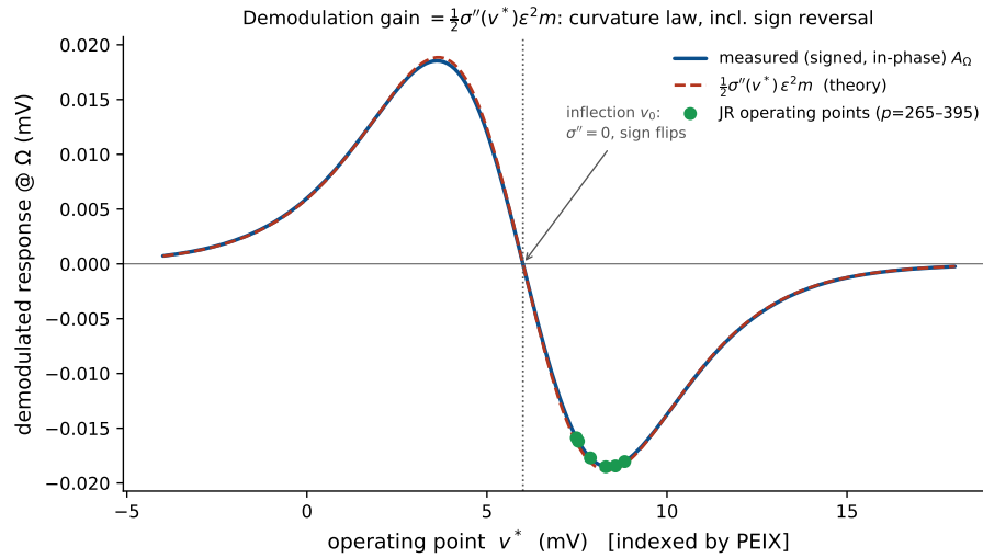
Figure 7: Operating-point law and the \sigma'' control (Jansen–Rit). The measured signed (in-phase) open-loop response tracks \frac{1}{2}\sigma''(v^*)\varepsilon^2 m across the whole range, vanishes at the inflection v_0 , and reverses sign across it—a direct verification that demodulation is the sigmoid-curvature term of Eq. (10). The closed-loop JR operating points (dots) sit on the lobe where \sigma'' is large and negative—not by design, but because that is where the JR resting point lies as the alpha Hopf is approached (the saturating upper flank of the sigmoid). The mechanism is sign-agnostic: \sigma'' sets only the sign/phase of the demodulated response while |\sigma''| sets its gain, so the entire resonance picture is unchanged (up to an overall sign) in the \sigma'' > 0 lobe, which this open-loop sweep already spans. The sign flip itself is a falsifiable prediction (§4.10).
