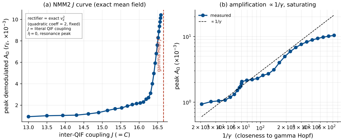
Figure 11: Coupling controls the amplification in the exact mean field (NMM2 PING, gamma). J ( = C ) is the literal inter-QIF synaptic weight; the rectifier is the exact v_E^2 (fixed quadratic coefficient), so no operating-point pinning is needed. (a) The peak demodulated response of r_E grows as J \rightarrow J^* (gamma Hopf, \bar{\eta} = 0 ; stable focus, \gamma > 0 ). (b) The gain grows as 1/\gamma (dashed), saturating near criticality—the JR law, now with coupling and rectifier both derived.
