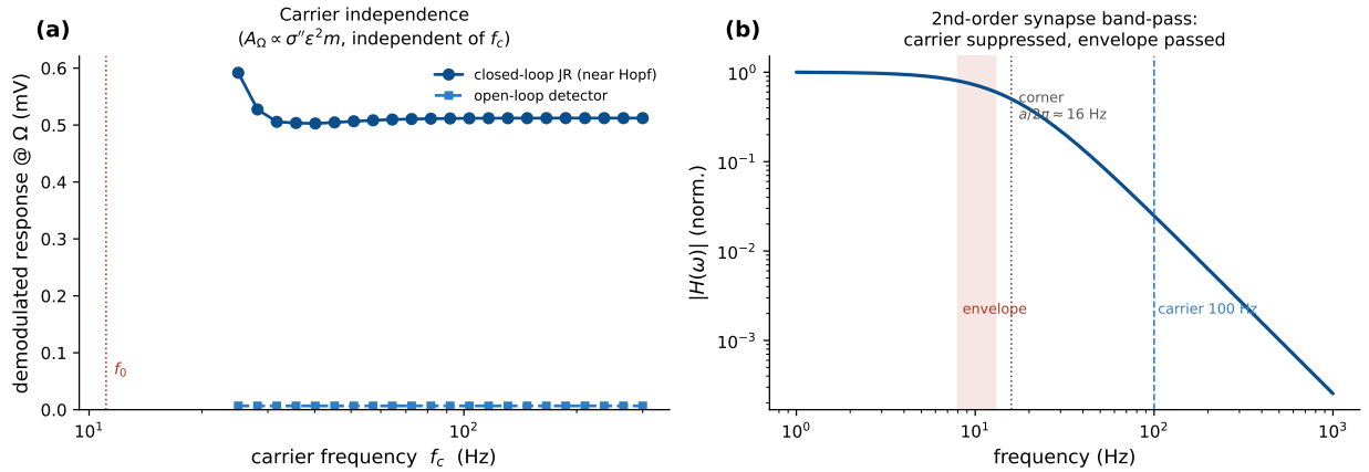
Figure 5: The demodulated response is carrier-independent at fixed polarization (Jansen–Rit). Left: the demodulated response is flat across carrier frequency f_c = 25 –300 Hz, both for the open-loop detector (exactly, by Eq. (10)) and for the closed-loop JR near the Hopf (which adds \sim 60\times resonant gain); deviations appear only as f_c approaches the natural band. Right: the second-order-synapse band-pass |H(\omega)| passes the envelope ( \sim 0.7 ) and suppresses the 100 Hz carrier ( \sim 2.5\% ).
