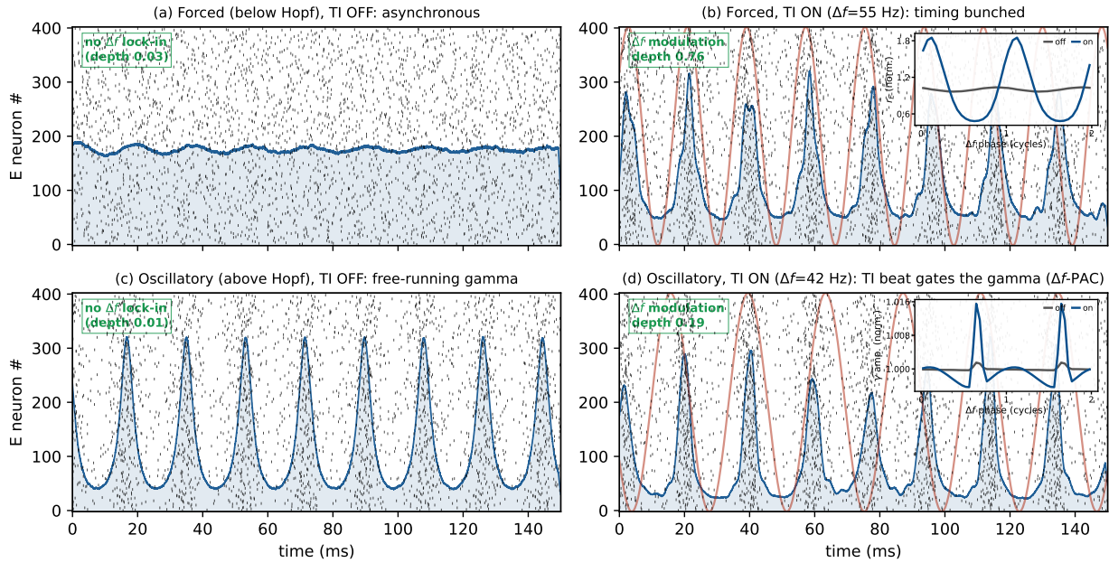
Figure 13: QIF spiking network (microscale of the NMM2 PING gamma generator): TI realigns spike timing, not mean rate. N = 8000 excitatory and inhibitory quadratic integrate-and-fire neurons whose exact mean field is the NMM2 PING circuit (Eq. (16)). This circuit’s intrinsic rhythm is gamma ( \sim 53 Hz), so—as in the alpha figures, but one band up—the TI beat \Delta f is set in the gamma range (here much larger than the \Delta f \sim 11 Hz of the Jansen–Rit alpha column; carrier f_c = 300 Hz). Black ticks are E spikes (400 of 8000, a representative sample), blue the population rate r_E(t) , red the TI envelope; the boxed value is the \Delta f modulation depth A_\Omega/\langle r_E \rangle of the rate (near zero off, large on). The bifurcation parameter is the common background drive \bar{\eta} (gamma Hopf at \bar{\eta}_{\text{Hopf}} \approx 1.1 ). (a) Forced ( \bar{\eta} = 0.85 , just below the Hopf—a damped gamma resonator), TI off: asynchronous firing, flat rate. (b) Forced, TI on, driven near the gamma resonance ( \Delta f = 55 Hz): spikes bunch into the envelope (modulation depth 0.76). (c) Oscillatory ( \bar{\eta} = 1.5 , above the Hopf—an autonomous \sim 53 Hz gamma cycle), TI off: free-running gamma, no \Delta f lock-in. (d) Oscillatory, TI on, with the beat set below the autonomous gamma (beat \Delta f = 42 Hz, a detuning of \approx 11 Hz from f_0 \approx 53 Hz): the TI beat gates the gamma—the population rate gains a \Delta f -locked component (modulation depth 0.19) while the intrinsic \sim 53 Hz gamma persists. This is forced cross-frequency gating (PAC), not frequency entrainment: the \sim 11 Hz detuning places the beat outside the 1:1 Arnold tongue (contrast the genuine frequency locking of Fig. S5), so the gamma is amplitude-modulated at \Delta f rather than pulled to it—demodulation surviving above the Hopf as envelope-to-rhythm coupling. The detuning is what certifies the \Delta f -locked component as a real driven effect rather than coincidence. Insets (each normalized to its own mean, so the y -axis reads the relative modulation; x -axis is the \Delta f beat phase in cycles; TI off gray, on blue): (b) the population rate folded on the beat phase (the forced response is at \Delta f ); (d) the gamma-band amplitude folded on the beat phase—taking the amplitude removes the gamma carrier, so the near-commensurate 53/42 Hz gamma cannot contaminate the fold (a raw-rate fold would). Both are flat with TI off and show a clear \Delta f -locked modulation with TI on, making the envelope-locked timing direct where the raster alone leaves it subtle.
