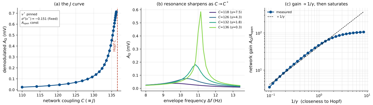
Figure 10: Coupling controls the amplification at fixed detection (Jansen–Rit). The operating point v^* is pinned by co-solving p(C) , so \sigma''(v^*) and A_{\text{open}} are constant. (a) The demodulated A_\Omega grows as the coupling C (= J) approaches the Hopf C^* from the stable-focus side ( \gamma > 0 ). (b) The envelope resonance sharpens and grows as C \rightarrow C^* . (c) The network gain A_\Omega/A_{\text{open}} follows 1/\gamma (dashed) and saturates near the bifurcation.
