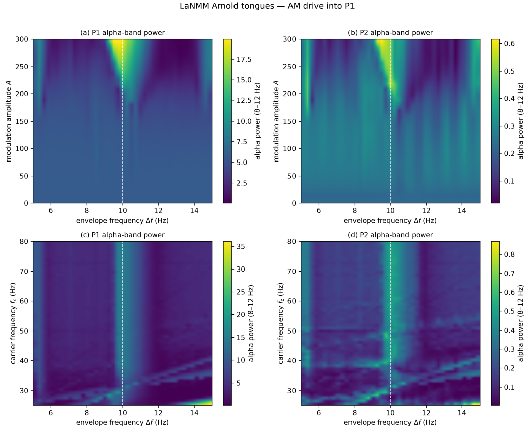
Figure S10: LaNMM Arnold tongues: AM input delivered directly to the deep P_1 (alpha) loop. (a,b) Alpha power of P_1 and P_2 vs. amplitude A and \Delta f . (c,d) Alpha power vs. carrier frequency and \Delta f : P_1 responds across a broad carrier band (a vertical ridge at \Delta f \approx 10 Hz)—carrier-independent, the direct-coupling limit of Eq. (10).
