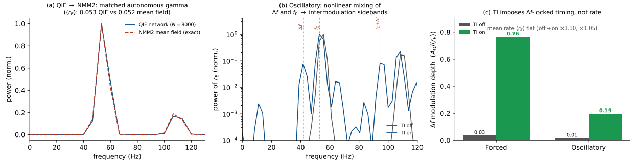
Figure 14: Timing, not rate, in the QIF network. (a) Power spectrum of r_E(t) in the field-free (autonomous) state: the spiking network ( N = 8000 ) matches the exact NMM2 mean field in the gamma rhythm (both \sim 53 Hz) and in mean rate \langle r_E \rangle . (b) Intermodulation in the oscillatory regime (TI off vs. on, log power): with TI on the nonlinearity mixes the imposed \Delta f = 42 Hz beat with the intrinsic f_0 \approx 53 Hz gamma, lighting up the direct \Delta f line and the sum sideband f_0 + \Delta f \approx 95 Hz, both absent when TI is off (the difference tone f_0 - \Delta f \approx 11 Hz sits near the floor, its amplitude set by the network transfer function rather than the mixer)—the spiking-network view of the same sigmoid frequency-mixing that drives demodulation throughout, and the sideband signature of gating rather than entrainment. (c) The \Delta f modulation depth A_\Omega / \langle r_E \rangle —the amplitude of the \Delta f -locked rate oscillation as a fraction of the mean rate—off vs. on: near zero with TI off (0.01–0.03), large with TI on (0.19 oscillatory, 0.76 forced), while the mean rate stays flat ( \times 1.05 – \times 1.10 ). We report the modulation depth rather than the off \rightarrow on lock-in ratio because the latter divides by the near-zero field-free baseline and is realization-noisy; the depth uses two well-estimated quantities and is stable.
