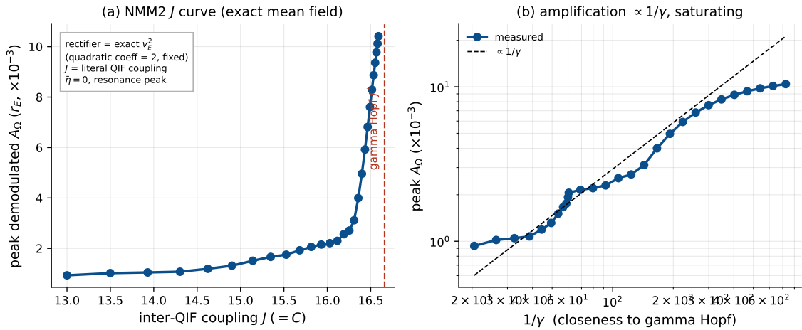
Figure S13: Coupling controls the amplification in the exact mean field (NMM2 PING, gamma). J (= C) is the literal inter-QIF synaptic weight; the rectifier is the exact v_E^2 (fixed quadratic coefficient), so no operating-point pinning is needed. (a) The peak demodulated response of r_E grows as J \rightarrow J^* (gamma Hopf, \bar{\eta} = 0 ; stable focus, \gamma > 0 ). (b) The gain grows as 1/\gamma (dashed), saturating near criticality—the JR law, now with coupling and rectifier both derived.
