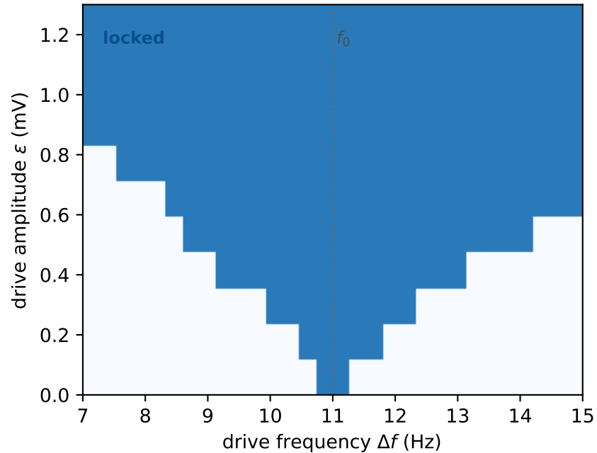
(a) Arnold tongue (one p )
