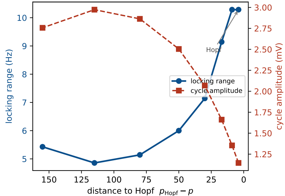
(c) entrainment grows toward criticality
