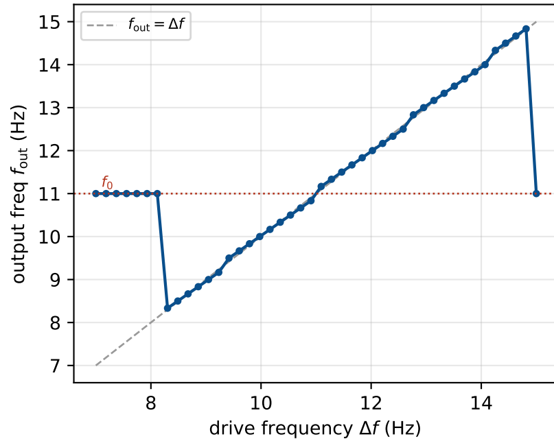
(b) frequency locking
