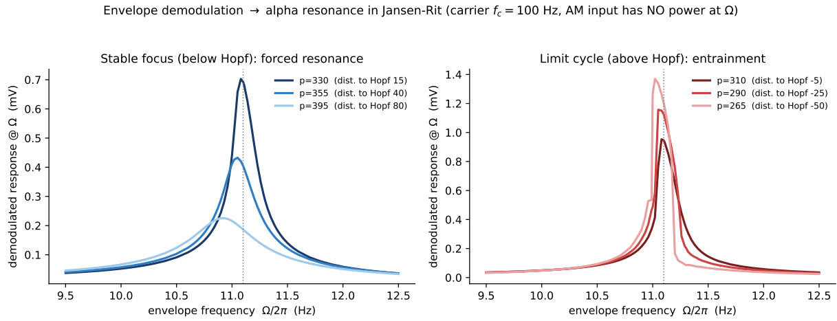
Figure 5: Resonance near vs. far from the Hopf (Jansen–Rit). Lock-in response at \Omega vs. envelope frequency ( \varepsilon = 0.3 mV). Left (stable focus, p > 315 ): forced resonance at f_0 \approx 11.1 Hz; the peak grows monotonically as p \rightarrow 315 , i.e. gain \propto 1/\gamma . Right (limit cycle, p < 315 ): the demodulated drive entrains the autonomous alpha rhythm.
