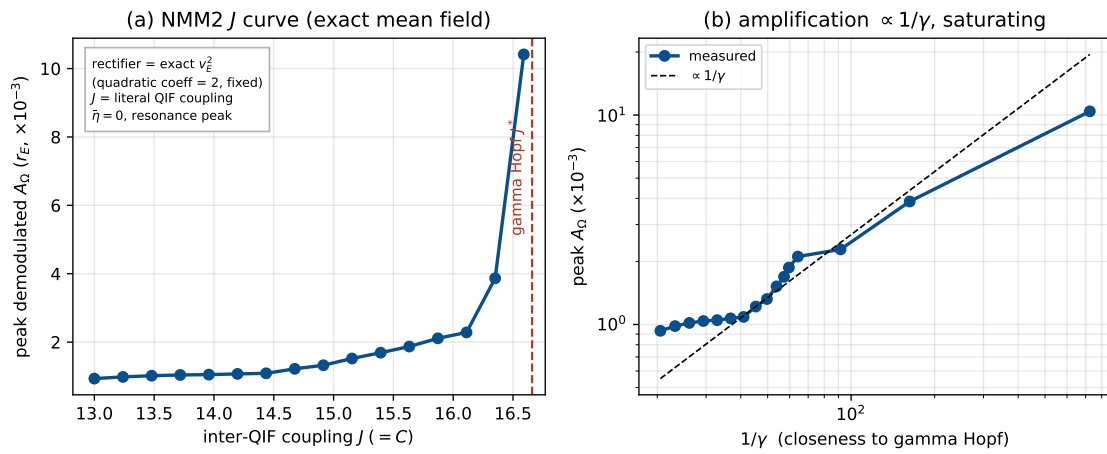
Figure 19: Coupling controls the amplification in the exact mean field (NMM2 PING, gamma). J (=C) is the literal inter-QIF synaptic weight; the rectifier is the exact v_E^2 (fixed quadratic coefficient), so no operating-point pinning is needed. (a) The peak demodulated response of r_E diverges as J \rightarrow J^* (gamma Hopf, \bar{\eta} = 0 ). (b) The gain grows as 1/\gamma (dashed), saturating near criticality—the JR law, now with coupling and rectifier both derived.
