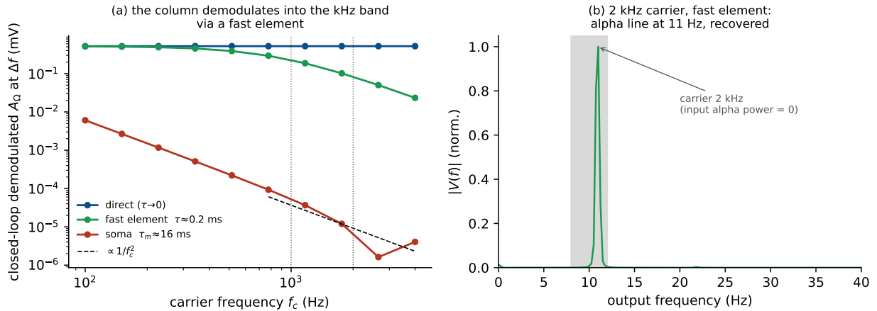
Figure 9: Demodulation at a genuine kHz carrier (Jansen–Rit, closed loop). The applied field passes through an explicit membrane filter before the sigmoid. (a) Closed-loop demodulated A_Q at \Delta f = f_0 vs. carrier f_c for three coupling routes: direct ( \tau \rightarrow 0 , carrier-independent), fast element (axon/AIS/node, \tau \approx 0.2 ms; survives into the kHz band), and soma ( \tau_m \approx 16 ms; collapses as 1/f_c^2 ). (b) Output spectrum for a 2 kHz carrier delivered through the fast element: a clean alpha line at f_0 , synthesized by the column although the input carries no alpha power.
