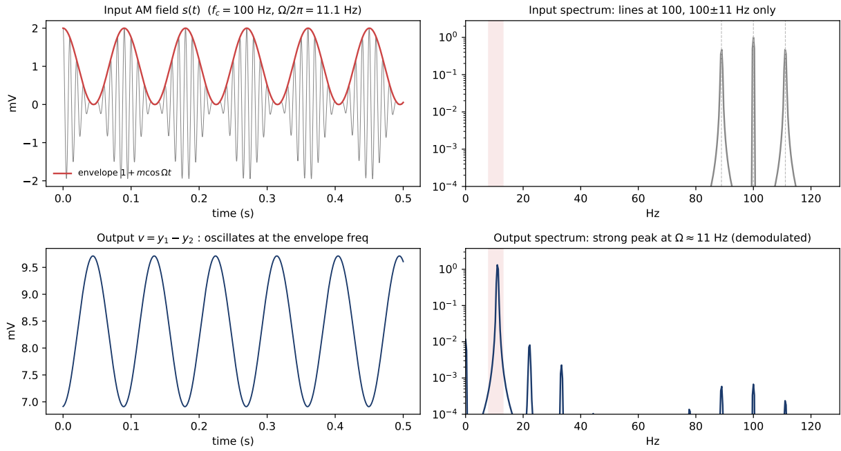
Figure 4: Demodulation in the Jansen–Rit column (proof of concept). Top left: the AM field s(t) and its envelope. Top right: the input spectrum has lines only at f_c and f_c \pm \Delta f (89, 100, 111 Hz); the alpha band (shaded) is empty. Bottom left: the output v = y_1 - y_2 oscillates at the envelope frequency. Bottom right: the output spectrum has a strong peak at \Omega \approx 11 Hz, synthesized by the sigmoid and absent from the input.
