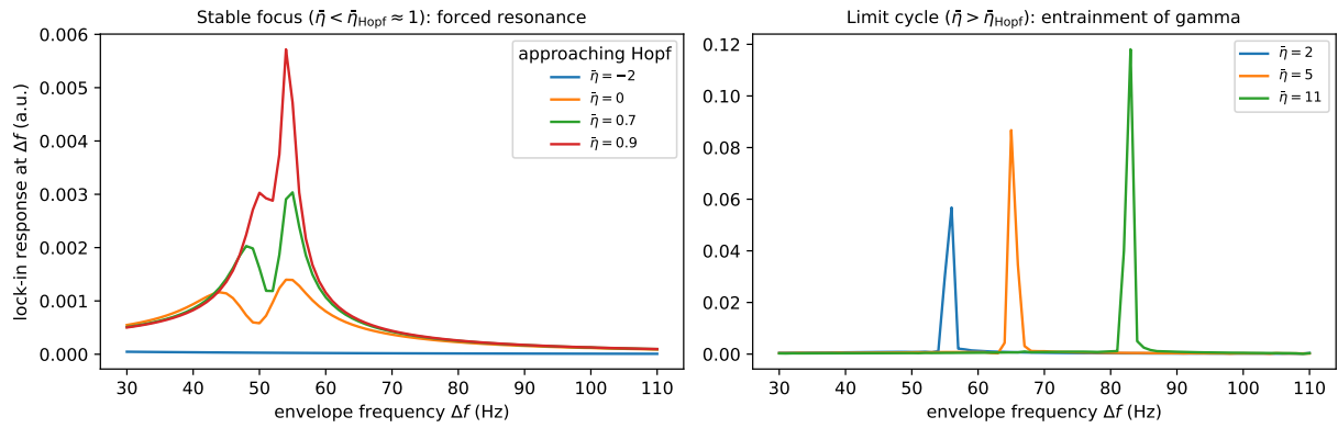
Figure 16: NMM2 PING gamma resonance (exact mean field). Lock-in response of the excitatory rate r_E at the envelope frequency \Delta f under an AM field (carrier 300 Hz). Left (stable focus, \bar{\eta} < \bar{\eta}_{\text{Hopf}} \approx 1 ): forced resonance at the gamma frequency ( f_0 \approx 55 Hz), growing as the Hopf is approached ( 1/\gamma gain), with the resonant frequency rising with \bar{\eta} . Right (limit cycle, \bar{\eta} > \bar{\eta}_{\text{Hopf}} ): entrainment of the autonomous gamma. The input carries no power at \Delta f ; the response is synthesized by the exact quadratic v^2 nonlinearity.
