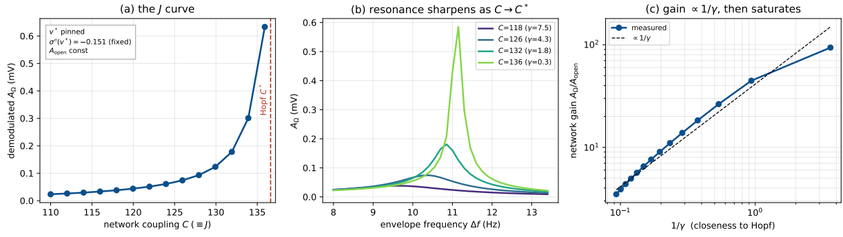
Figure 18: Coupling controls the amplification at fixed detection (Jansen–Rit). The operating point v^* is pinned by co-solving p(C) , so \sigma''(v^*) and A_{\text{open}} are constant. (a) The demodulated A_\Omega diverges as the coupling C (=J) approaches the Hopf C^* . (b) The envelope resonance sharpens and grows as C \rightarrow C^* . (c) The network gain A_\Omega/A_{\text{open}} follows 1/\gamma (dashed) and saturates near the bifurcation.
