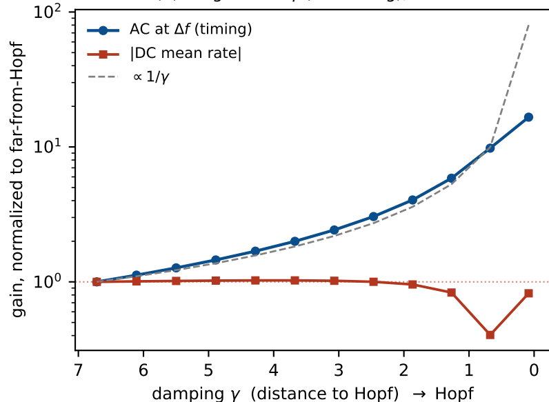
(b) AC gain \sim 1/\gamma (saturating); DC flat
